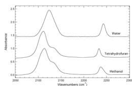
Figure 1. FTIR absorbance spectra of \text{N}_3\text{CNDU} dissolved in water, tetrahydrofuran (THF), or methanol recorded at 293 K with a concentration of 50 mM. The maximum absorbance of each spectrum has been normalized to unity and the spectra have been offset for comparison.
