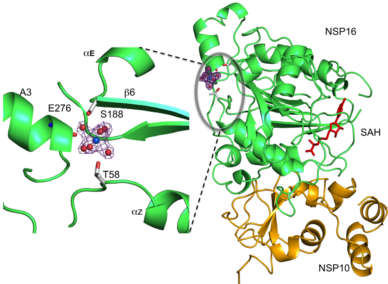
Figure 4. Position and coordination of a metal ion. Left, the putative Mg^{2+} ion (blue sphere) is shown solvated in its first atomic shell by six water molecules (red spheres). The corresponding 2F_o-F_c electron density map (contoured 1\sigma ) with a cross shape is shown in purple. Residues of Nsp16 involved in coordination of Mg^{2+} ion via water molecules are labeled. Right, a global view of the bound metal ion in its electron density on the opposite side from the SAH molecule (red sticks). Nsp16 is shown as green ribbons, nsp10 as yellow ribbons with its two bound Zn^{2+} as grey spheres as in Fig. 1.
