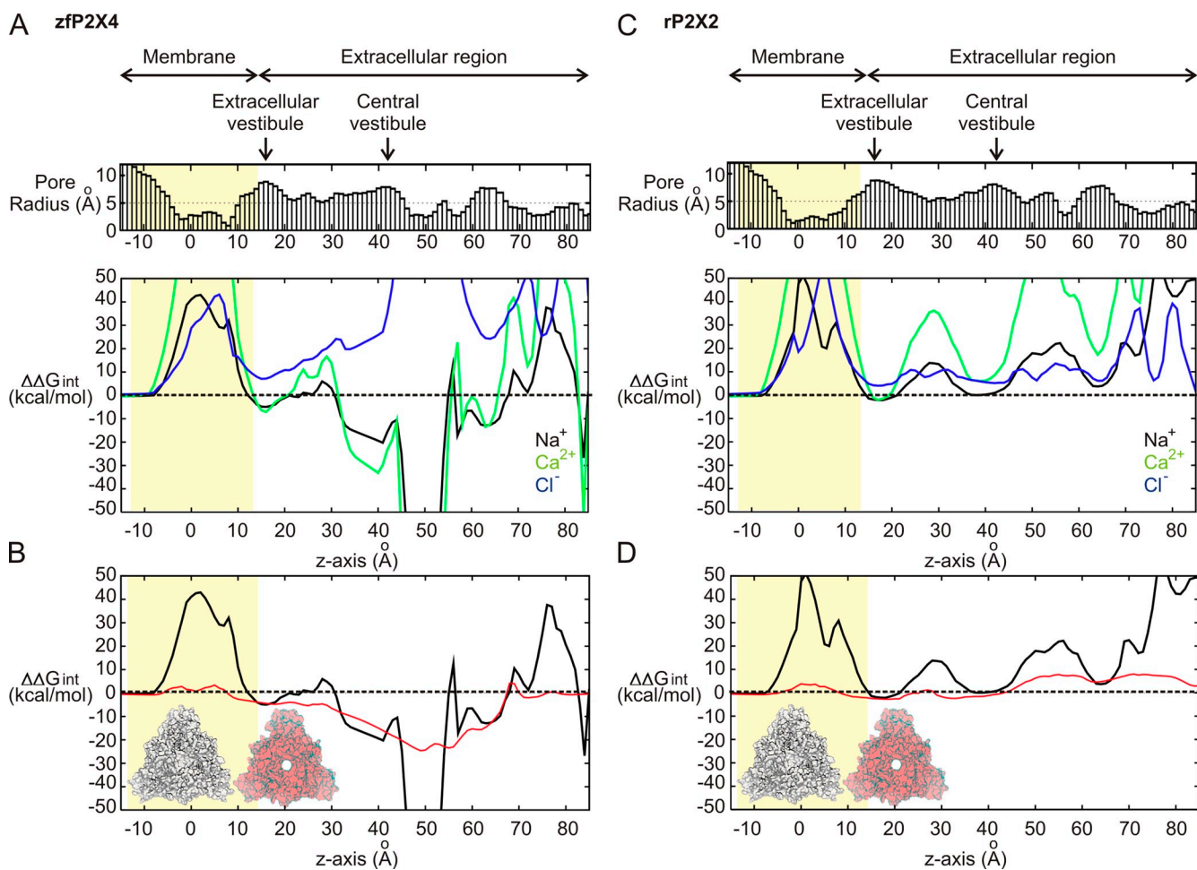
Figure 2. Electrostatic interaction free energy of ions along the central pathways in zP2X4 and rP2X2. Results for zP2X4 are shown in A and B, whereas those for rP2X2 are shown in C and D. (A and C) \Delta\Delta G_{\text{int}} of \text{Na}^+ (black), \text{Ca}^{2+} (green), and \text{Cl}^- (blue), calculated along the central pathway, with the transmembrane region depicted with the yellow slab and the center of the membrane at Z = 0 Å. The pore radius profile is shown in the bar graph on top. (B and D) \Delta\Delta G_{\text{int}} of \text{Na}^+ along the central pathway of the original closed model (black), and an artificially opened pore widened to 5-Å radius from the molecular threefold symmetry axis (red). The surface representations of the original closed (white) and the forced open (red) conformations are shown.
