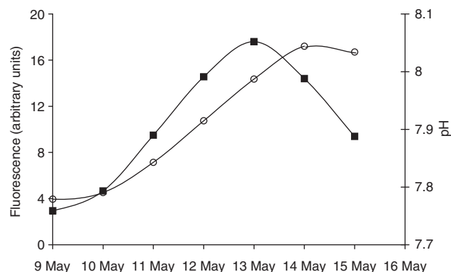
Figure 1 Rapid change in pH (○) as phytoplankton biomass (■) increased during a bloom in a mesocosm experiment (Gilbert et al. , 2008). Water had been bubbled with \text{CO}_2 -enriched air (750 \mu\text{atm} ) and the bloom was initiated by the addition of nitrate and phosphate. The mesocosm was covered and there was no exchange of \text{CO}_2 with the atmosphere; the observed changes in pH were the result to the utilization of dissolved \text{CO}_2 by the actively growing phytoplankton assemblage.
