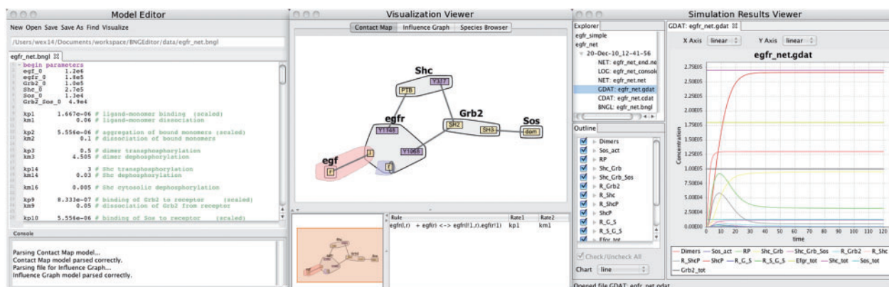
Fig. 1. The RULEBENDER interface with Model Editor window including Console for simulation (left), a Visualization Viewer window (middle) and a Simulation Results Viewer window (right). RULEBENDER's main features include syntax checking, syntax highlighting, visual global model exploration, integrated execution, support for multiple simulation modules, simulation journaling, interactive plotting including comparison of multiple datasets and parameter scanning.
