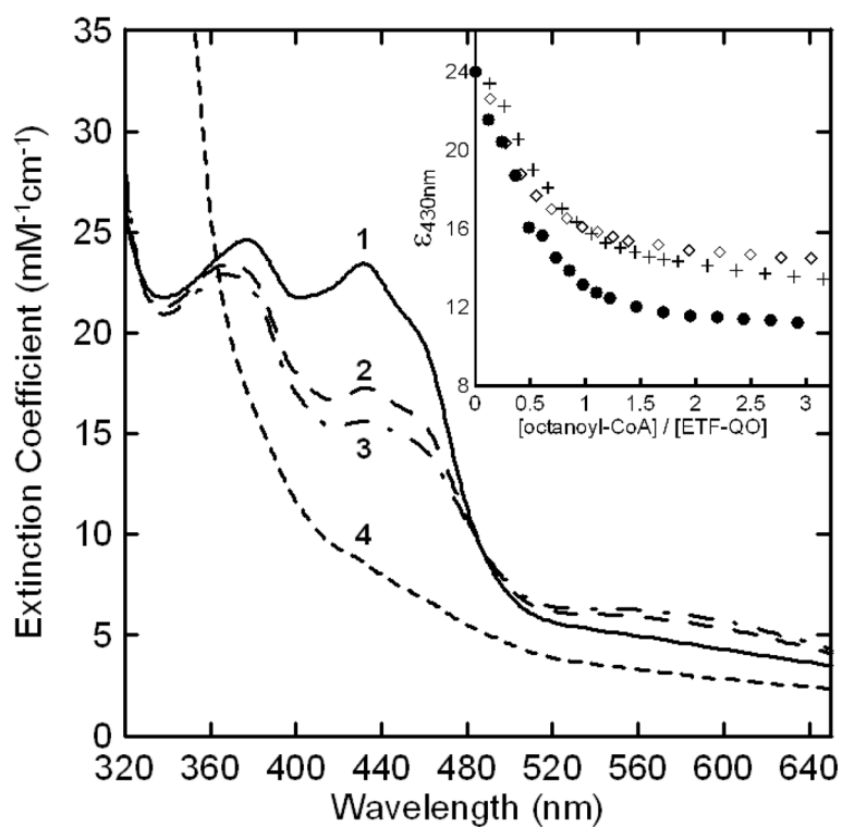
Figure 3. Anaerobic reductive titration of N338A ETF-QO. The solution contained 20 \mu\text{M} R. sphaeroides N338A ETF-QO, 1.5 \mu\text{M} human ETF, and 0.5 \mu\text{M} human MCAD in 10 mM Hepes(K + ) at pH 7.4. The oxidized sample (spectrum 1) was titrated with octanoyl-CoA. After each addition spectra were recorded every 5–10 minutes until less than 0.001 a.u. change per minute in absorbance was observed. Spectra 2 and 3 correspond to mole ratios of 0.5:1 and 1:1, respectively, and spectrum 4 is the dithionite reduced enzyme. The inset shows the \Delta\epsilon_{430\text{ nm}} vs. mole ratio of titrant for (●) wild type, (+) N338T, and (◇) N338A ETF-QOs.
