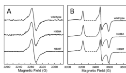
Figure 4. X-band CW EPR spectra of R. sphaeroides ETF-QO. (A) FAD semiquinone signal recorded at 100 K, 9.23 GHz with 0.01 mW power. A similar lineshape, but with lower signal-to-noise, was observed at 293 K. (B) [4Fe-4S] + signal recorded at 15 K, 9.35–9.42 GHz with 0.05 mW power. The saturated FAD semiquinone signal was deleted from (B) to aid in comparison (dashed lines). The anaerobic samples contained 20 mM Hepes and 20% glycerol (v/v) at pH 7.4. Spectra were recorded at their respective maximum semiquinone signals from the potentiometric titrations. The potentials were: wild type (–10 mV), N338A (–75 mV), and N338T (–35 mV).
