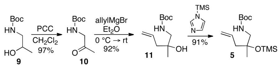
Scheme 2. Synthesis of Carboamination Substrate
