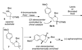
Scheme 1. Asymmetric Carboamination/Friedel-Crafts Alkylation Strategy
