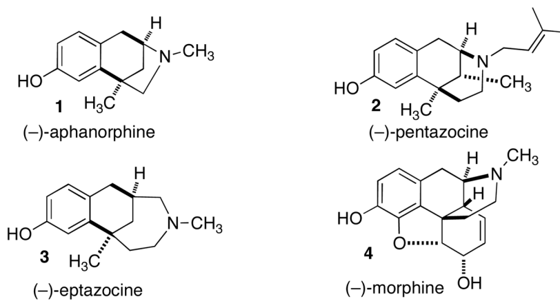
Figure 1. Benzomorphan Alkaloids
