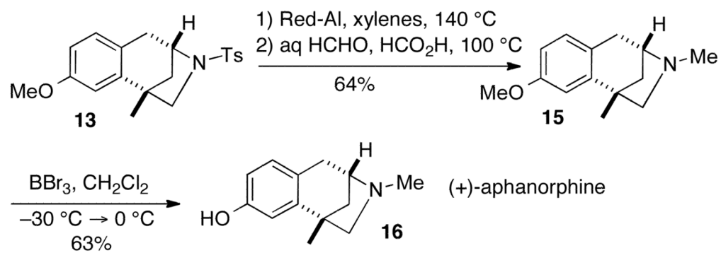
Scheme 4. Completion of the Synthesis
