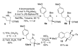
Scheme 3. Pd-Catalyzed Carboamination of 5 and Conversion to 13 .
