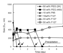
Fig. 1. Particle size of pH-sensitive micelles with excipients: 50 wt% PEG (2k) (◆), 50 wt% PEG (400) (■), 10 wt% P85 (▲), 10 wt% F127 (×), 33 wt% F127 (○), 50 wt% F127 (□); as a function of time. The 0 nm of particle size (arrows) indicates the precipitation of particle observed visually.
