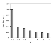
Fig. 2. Particle size of pH-sensitive micelles with F127 at various pHs. From pH 8.0 to 7.0 unimodal particle distribution and below pH 7.0, bimodal particle distributions were observed, respectively.
