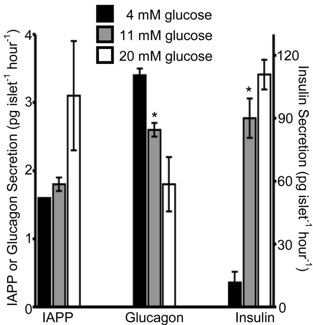
Figure 3. IAPP, glucagon, and insulin secretion in response to varying glucose levels Batches of 14 islets were incubated in 4 (black bars), 11 (grey bars), and 20 (white bars) mM glucose and the levels of IAPP, glucagon, and insulin secretion were measured after 6 hours of incubation. Average values are plotted ( n = 4 ) with error bars corresponding to \pm 1 standard error of the mean. IAPP and glucagon values are shown on the left y-axis and insulin values are shown on the right y-axis.. * = p < 0.05 .
