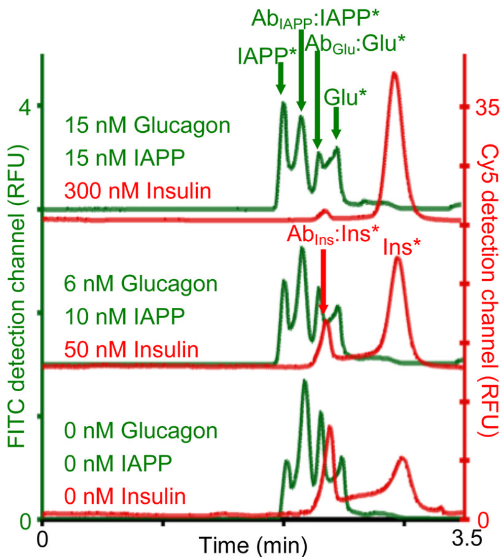
Figure 1. Simultaneous electropherograms of IAPP, glucagon, and insulin
