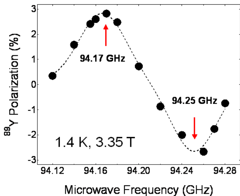
Figure 1. ^{89}\text{Y} polarization of the yttrium complex of 1,4,7,10-tetraazacyclododecane-1,4,7,10-tetraacetic acid (DOTA) (0.28 M in 1:1 vol/vol glycerol:water doped with 15 mM OX063 trityl radical) as a function of microwave frequency. The up and down arrows indicate the positive and negative polarization peaks, respectively. Each datapoint represents a separate DNP experiment.
