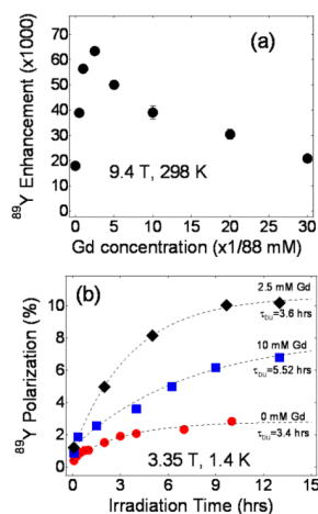
Figure 3. Effect of Gd(III) doping. (a) Room-temperature liquid-state NMR enhancement as a function of Gd doping in the solid-state. The dilution factor of the Gd concentration after dissolution is 1/88. Maximum enhancement is achieved with 2.5 mM Gd doping. Each datapoint represents an average of three separate DNP experiments. (b) Polarization buildup curves of 0.28M YDOTA samples in 1:1 glycerol:water glassing matrix doped with 15 mM trityl and Gd (0 mM, 2.5 mM, 10 mM). Each datapoint represents a separate DNP experiment.
