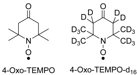
Chart 2. Free radical polarizing agents used in this work.
