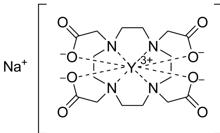
Chart 1. Structure of YDOTA
