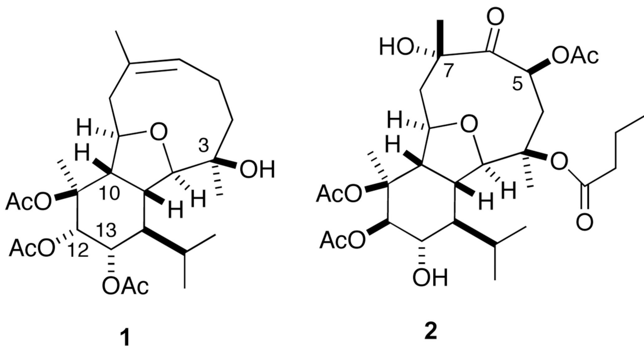
Figure 1. Massileunicellin C (1) and simplexin F (2).
