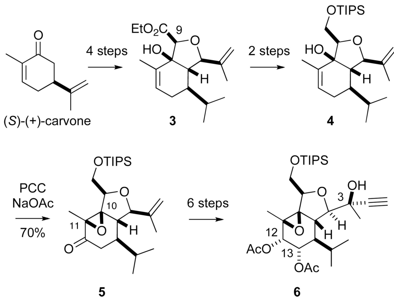
Scheme 1. Initial approach toward the massileunicellins.
