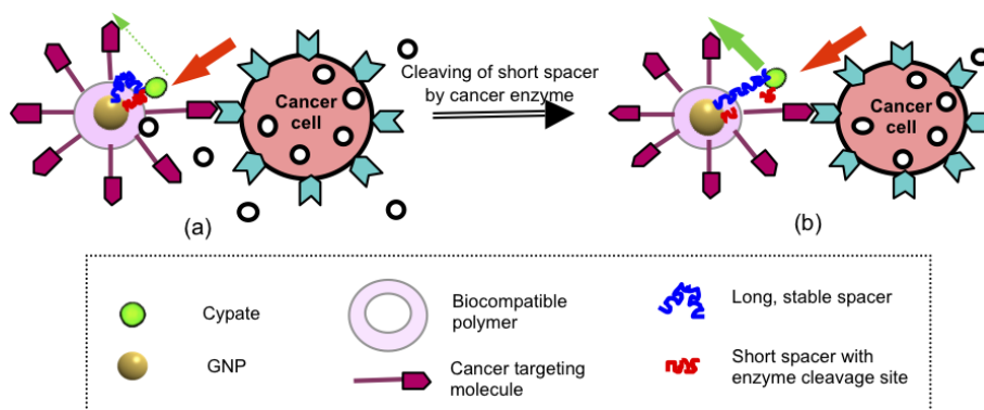
Figure 14 Design of a highly specific and sensitive optical contrast agent using GNP. (a) The cancer targeting molecule (red arrow) reacts with the receptor on the cancer cell; (b) The short spacer is cleaved by a cancer enzyme (o) and then the distance between Cypate and the GNP assumes the length of the long spacer, resulting in enhanced fluorescence.
