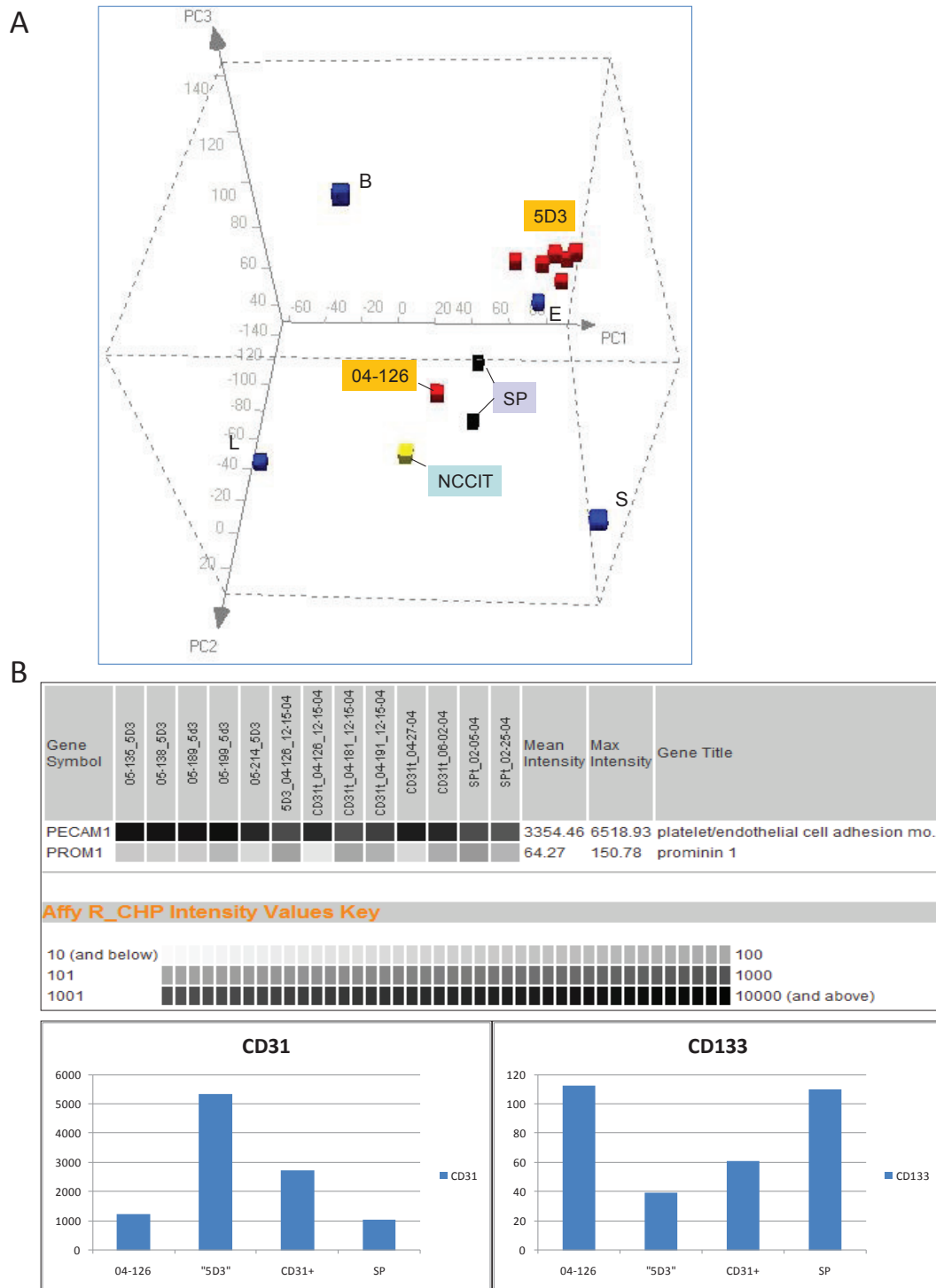
Figure 1 Principal components analysis of prostate ABCG2 + cells. A: This human prostate PCA space is keyed on the transcriptomes of B, L, S, and E cells. Stem cell transcriptome is represented by that of NCCIT. Putative progenitor cells sorted from the prostate by antibody to ABCG2 (clone 5D3) or in SP are shown. Many 5D3 sorts (red cubes) are found to cluster near E except for that derived from specimen 04-126. This and two SPs are positioned nearer the NCCIT. B: The expression levels of CD133 and CD31 in 04-126, other 5D3 sorts (labeled as "5D3"), endothelial sorts (labeled as CD31+) and SP are indicated by array signal values on a gray scale in the data query display. The histograms below show the same query output. Note the different expression magnitude scales on the y-axis for the two genes.
