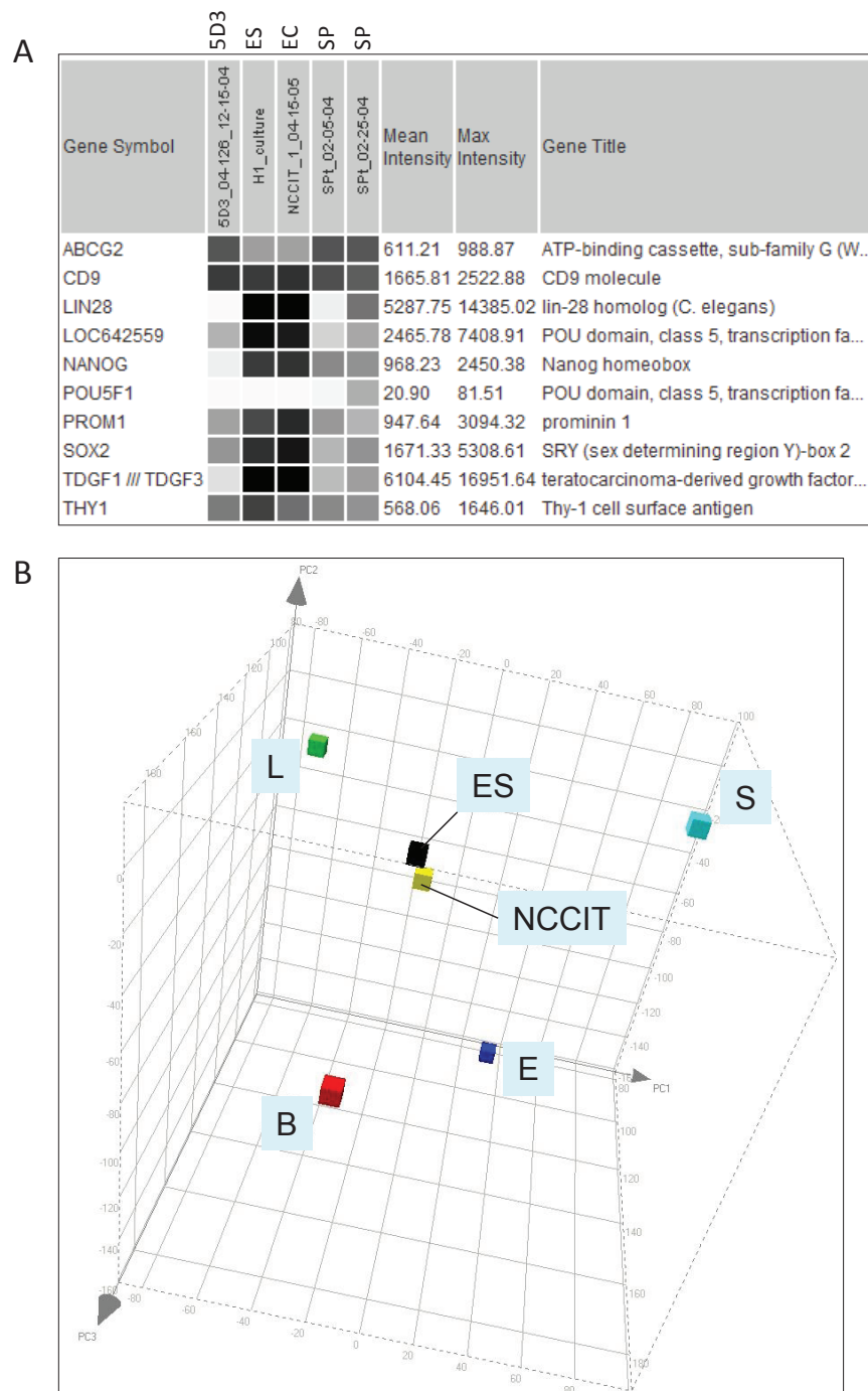
Figure 2 Gene expression comparison of ABCG2 + cells and stem cells. A: Differential expression of selected genes between 5D3 (04-126), SP and ES (H1) and EC (NCCIT) cells as obtained from dataset query is shown. B: PCA plot of H1 and NCCIT shows the close relatedness between these two cell types.
