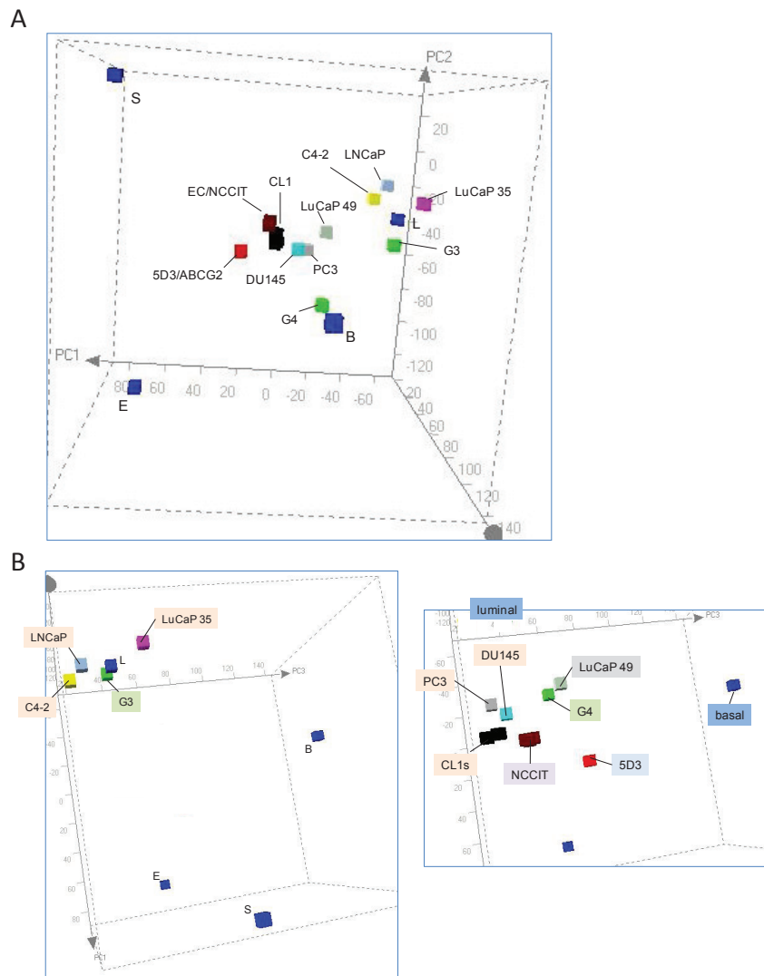
Figure 4 PCA of prostate cancer cell types. A: Transcriptomes of prostate primary cancer G3, G4, cell lines LNCaP, C4-2, CL1, DU145, PC3, xenografts LuCaP 35, LuCaP 49 are projected into the space defined by B-L-S-E. The CL1 data point also contains transcriptomes from CL1 subclones. B: Panel A shows grouping of the so-called luminal-like cancer cell types, while panel B shows grouping of the non-luminal-like cancer cell types in a different viewing aspect.
