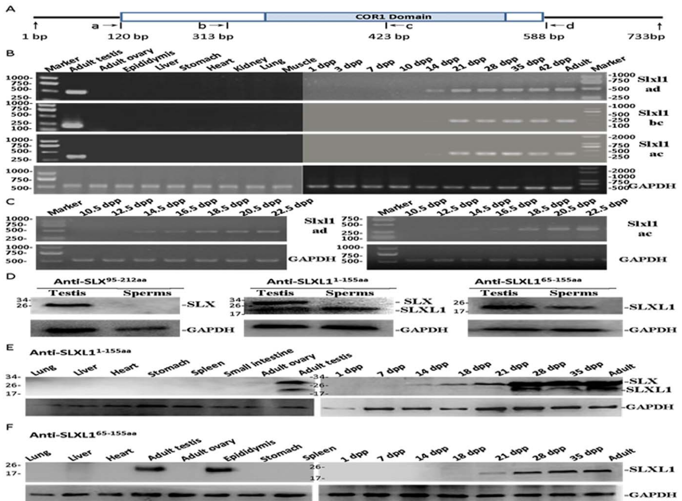
Figure 2. mRNA and protein expression of Slx1 in mouse tissues. (A). Positions of primers used in RT-PCRs. (B) Slx1 mRNA was exclusively expressed in mouse testes indicated by RT-PCR analysis of multiple tissues; Slx1 transcript was first detected at 14 days post partum (dpp) in postnatal mouse testes. (C) From 10.5 dpp to 22.5 dpp, Slx1 transcript level increased gradually as detected by RT-PCR using the ad and ac primer sets. (D) One protein of about 25 kDa in adult testis was detected in Western blotting, however, the protein was not detected in the spermatozoa using anti-SLX 95-212aa antibody. Using anti-SLXL1 1-155aa , two proteins of about 25 kDa and 18 kDa were detected in testes, while only the 18 kDa one was detected in spermatozoa. Only the 18 kDa protein was detected in either testis or spermatozoa using anti-SLXL1 65-155aa . (E–F) The expression of SLX and SLXL1 in mouse tissues and testes of different days post partum were detected using anti-SLXL1 1-155aa (E) and anti-SLXL1 65-155aa (F). mRNA and protein expression of GAPDH were used as internal controls for RT-PCR and Western Blot, respectively. doi:10.1371/journal.pone.0020866.g002
