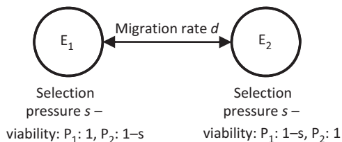
Fig. 1 A simple formal model of selection-based and detection-based effects. A population with two phenotypes P_1 and P_2 is split into two subpopulations living in environments E_1 and E_2 under selection pressure s against nonmatching phenotypes, and migrating between patches at rate d .
