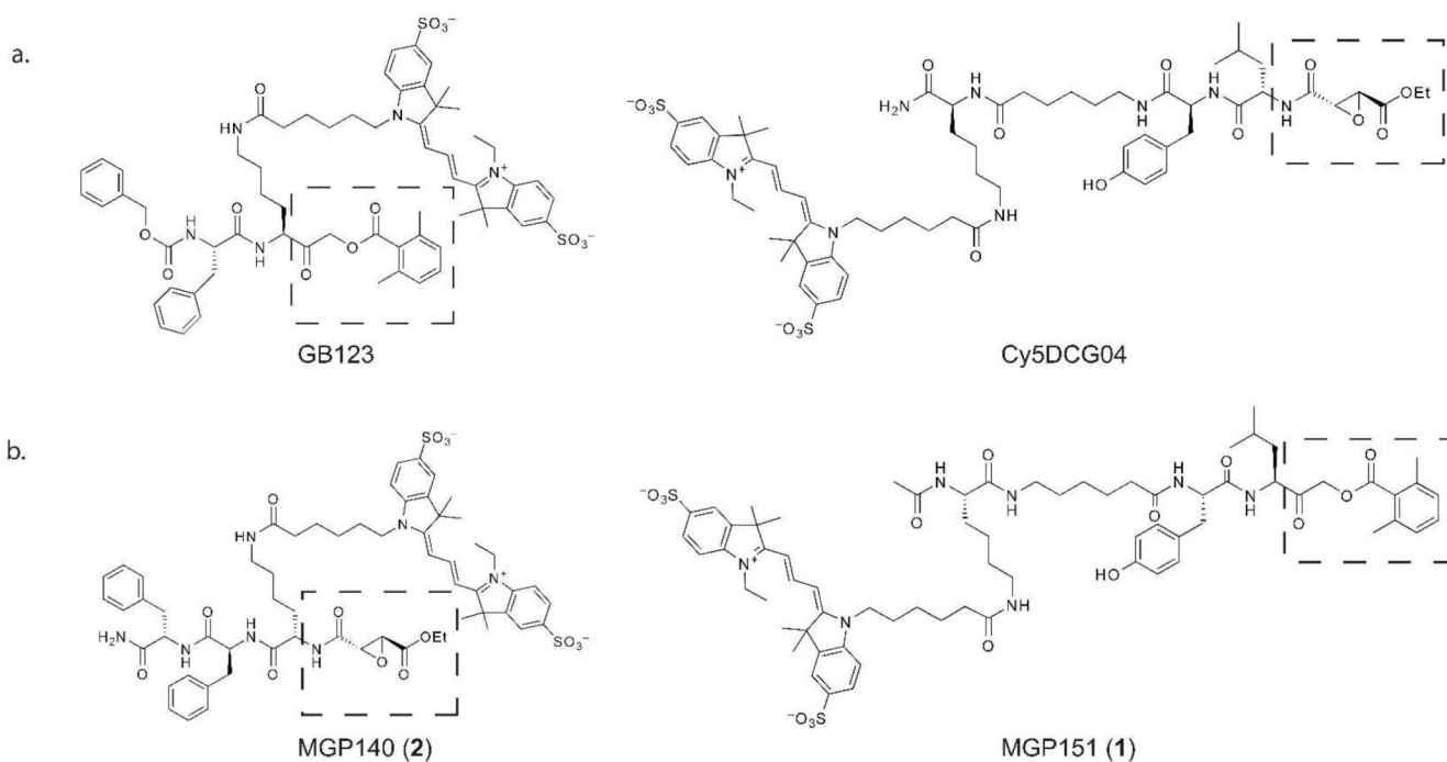
Figure 1. Structures of cysteine cathepsin activity-based probes
