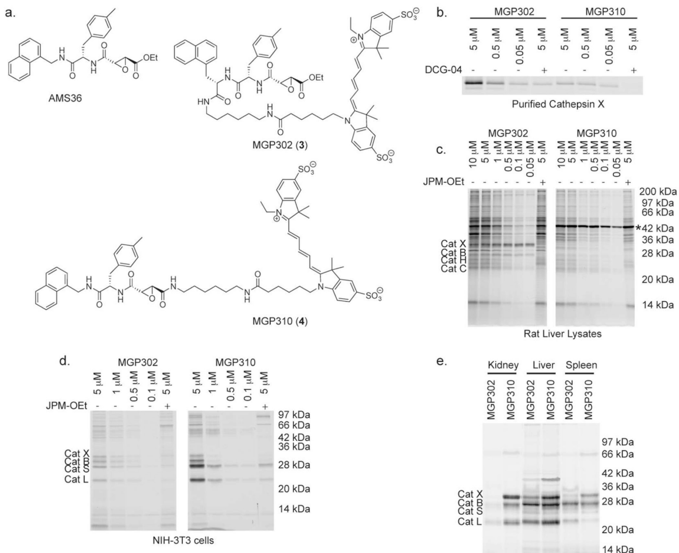
Figure 4. Structures and labeling selectivity of MGP302 and GP310
