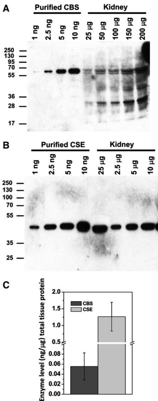
FIG. 3. Quantitative Western blot analysis of the transsulfuration pathway enzymes in kidney. Representative Western blot in which the indicated amounts of kidney extract were separated in parallel with known amounts of CBS (A) or CSE (B). Quantitation of CBS and CSE protein levels in kidney (C).
