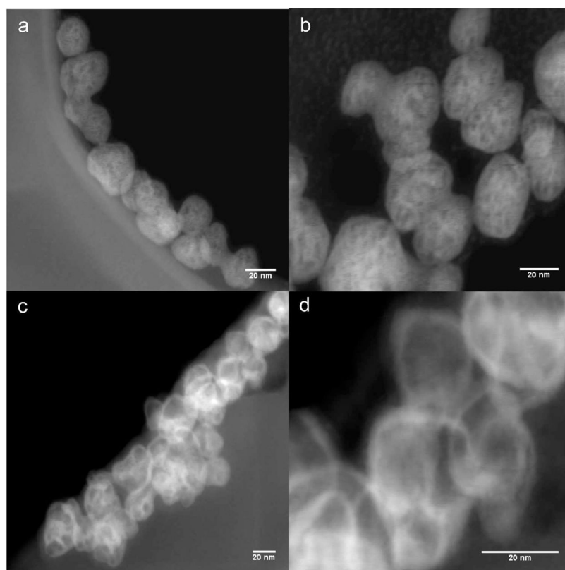
Figure 1. HAADF-STEM micrographs of uncoated cubic- \text{NaYF}_4 : 20% Yb: 2%Er nanophosphors (a and b). Core-shell architecture of the gold coated nanophosphors is shown in c and d. The gold shell is visible as bright contour in c and d.
