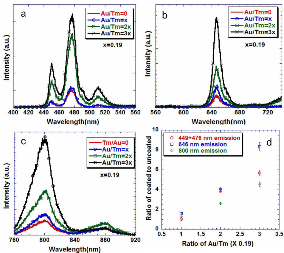
Figure 4. Up-converted emission from particles prepared with 0.1% solutions with different gold coatings on cubic \text{-NaYF}_4: 20\% \text{Yb}: 1\% \text{Tm} (a, b and c). d) Integrated area of the emission spectra from gold coated normalized to the uncoated nanophosphor. All solutions were excited at 975 nm.
