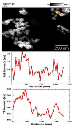
Figure 2. HAADF-STEM images and the EDS line spectra of Au and Y L-lines from gold coated cubic- \text{NaYF}_4 nanophosphors. Line in the STEM image indicates a transect across three particles, with corresponding profiles of Au and Y concentration shown below. The profile of Au and Y L-line from the particles show a close correspondence that indicates the association of Au with the Y based phosphor.
