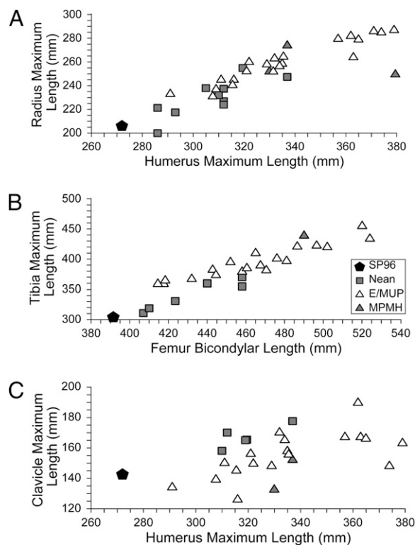
Fig. 2. (A–C) Bivariate plots of radius length versus humerus length (A), tibia length versus femur length (B), and clavicle length versus humerus length (C) ( SI Appendix, Tables S2 and S8 for individual lengths and SI Appendix, Table S9 for residual comparisons). SP96, Palomas 96; Nean, MIS 5d-3 Neandertals; E/MUP, MIS 3 Early/Mid-Upper Paleolithic modern humans; MPMH, MIS 5c Middle Paleolithic modern humans.
