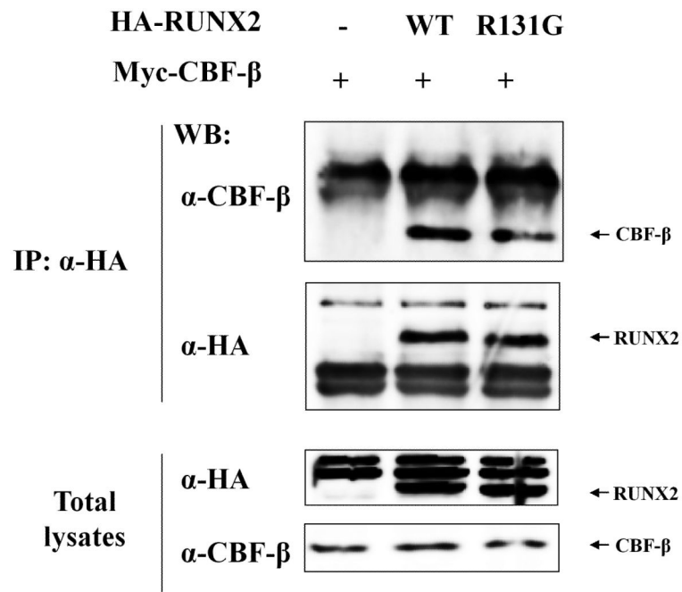
Figure 2. Heterodimerization of RUNX2 R131G with CBF- \beta HA tagged RUNX2 or RUNX2 R131G and Myc tagged CBF- \beta plasmid were co-transfected in HEK293 cells and proteins were immunoprecipitated with antibodies to HA. Immunoprecipitated proteins or total lysates were separated in 10% SDS-polyacrylamide gels, transferred, and immunoblotted with antibodies to either CBF- \beta or HA. -: Mock Plasmid; WT: HA tagged Wild Type RUNX2 plasmid; R131G: HA tagged RUNX2 R131G plasmid.
