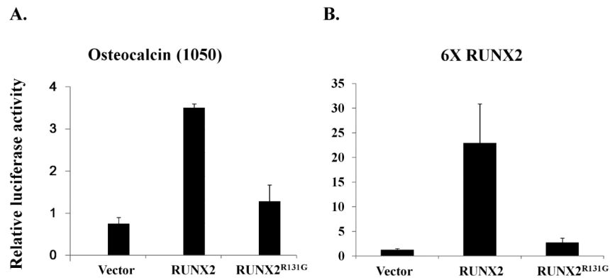
Figure 4. Trans-activation of RUNX2 or RUNX2 R131G
