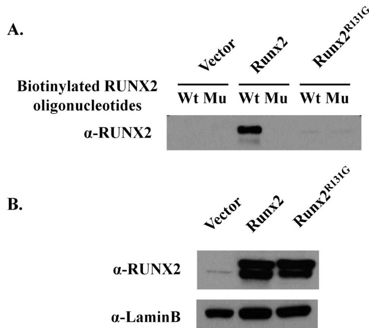
Figure 3. DNA binding activity of RUNX2 or RUNX2 R131G
