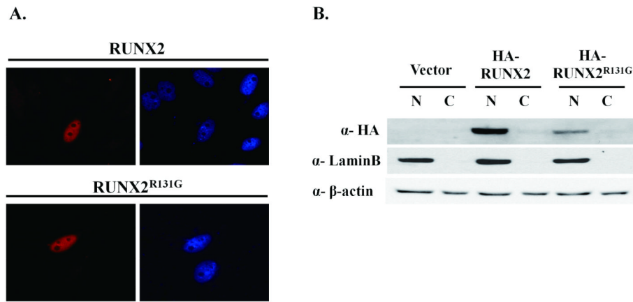
Figure 1. Subcellular localization of RUNX2 and RUNX2 R131G
