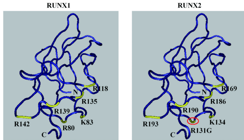
Figure 5. Three-dimensional structure of RUNX1 and RUNX2 runt domain
