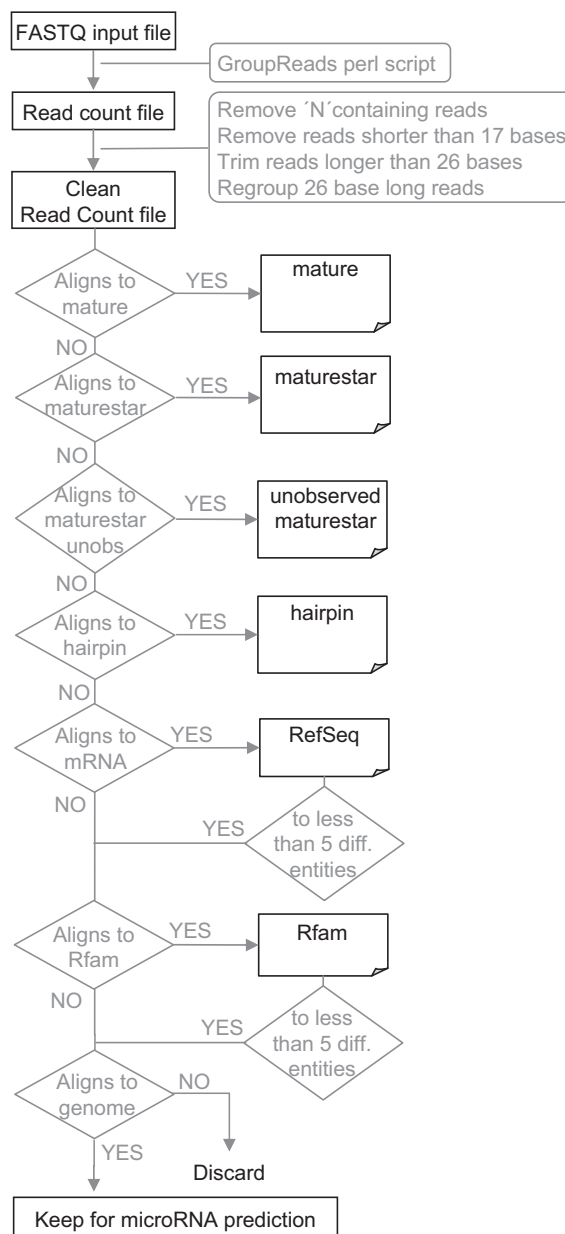
Figure 1. General workflow of miRanalyzer. The fastq file is transformed into a read count file, which is filtered to keep only sequences from 17 to 26 bases. These reads are successively mapped to several databases in order to identify known microRNAs, discard messenger RNA contaminations and select sequences for the microRNA prediction step.
