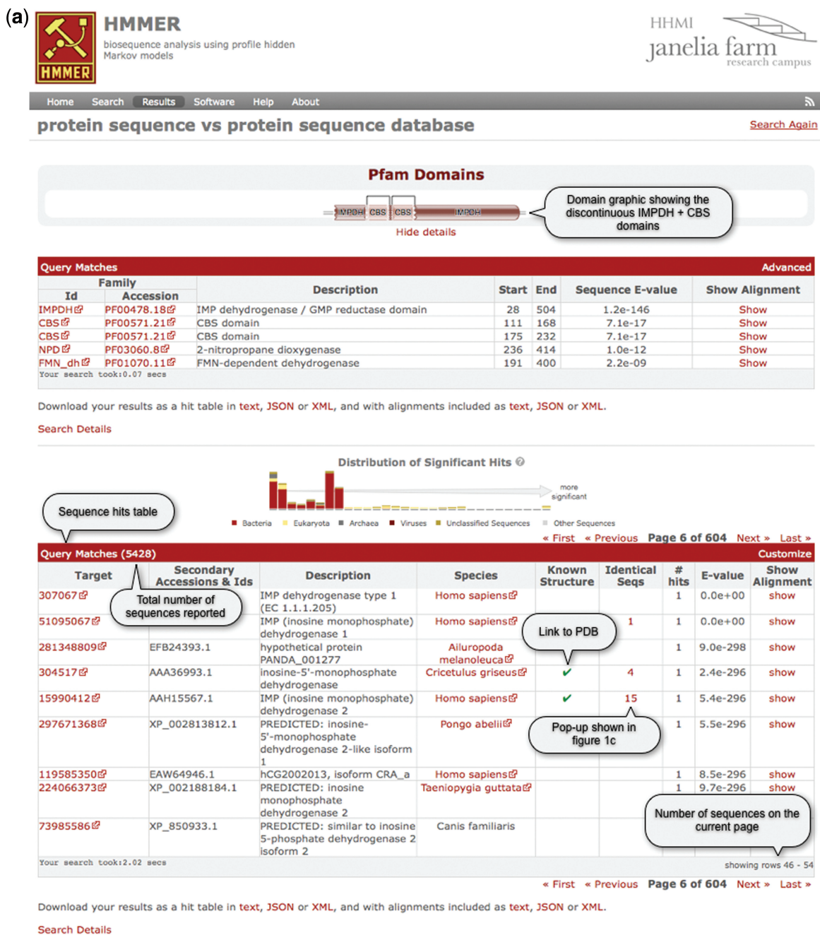
Figure 1. (a) A screen shot of the phmmer search results page, using the sequence IMDH1_HUMAN (UniProtKB) and default parameters. The results from the 'Pfam search' are shown as both a graphic and as a table, which has been revealed in this figure. Below this is a hit distribution graph and a table of the results from the phmmer search. Key features in the table are labeled and discussed in the text. This search resulted in over 5000 sequence matches, which are accessible either by going through the paginated table or can be navigated using the hit distribution histogram. (b) An enlarged version of the hit distribution graph, showing the taxonomic ranges of sequences matched in the search. The tool tip indicates the E -value range represented by the bar, and the number of sequences from the search that fall within the range.
