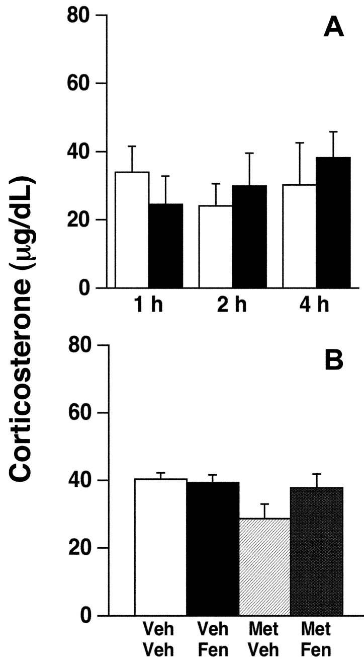
Fig 3. Plasma corticosterone levels following fenfluramine administration. No significant effects were noted in corticosterone levels after A ) PVN fenfluramine administration (200 nmol/0.5 µl/side; black bars = fenfluramine; white bars = vehicle) or B ) following metergoline (MET; 15 nmol/0.5 µl/side) and/or fenfluramine (FEN) administration compared to vehicle (VEH). n = 4-5/group.
