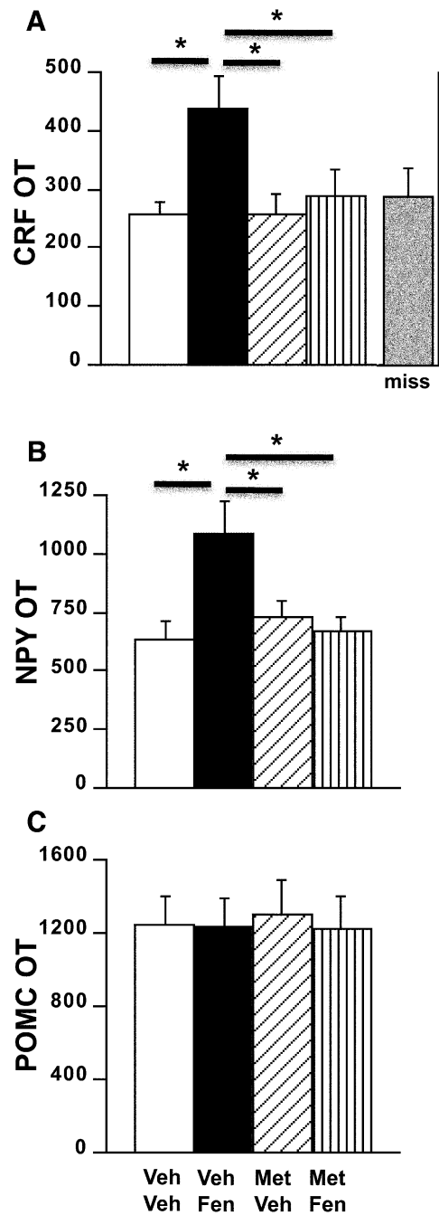
Fig 5. Hypothalamic neuropeptide mRNA levels following drug administration. Dark field analysis of silver grains expressed as levels of optical transmission (OT) of A ) CRF mRNA in the PVN (ANOVA, main treatment effect p < 0.02 ), B ) NPY mRNA in the arcuate nuclei (ANOVA, main treatment effect p < 0.02 ) and C ) POMC mRNA in the arcuate nuclei 1 hour after an acute injection of fenfluramine (FEN; 200 nmol/0.5 \mu l/side) and/or metergoline (MET; 15 nmol/0.5 \mu l/side). Miss = animals treated with fenfluramine but with incorrect cannulae placement. VEH = vehicle. * = p < 0.03 (Fisher's test); n = 4-5 /group.
