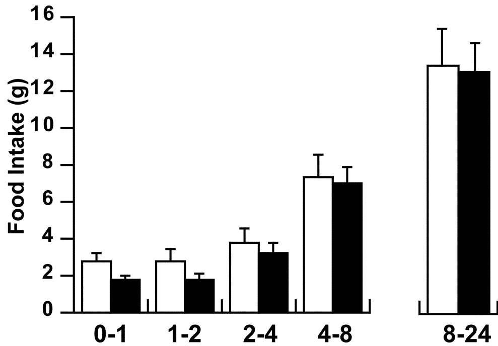
Fig 1. Time course of food intake following an acute injection of fenfluramine into the hypothalamic PVN. Feeding was suppressed 2 hours immediately after drug administration (ANOVA with repeated measures, p < 0.02 treatment; p < 0.0001 time). Black bars = fenfluramine (200 nmol/0.5 \mu l/side); white bars = vehicle. n = 8-10 /group
