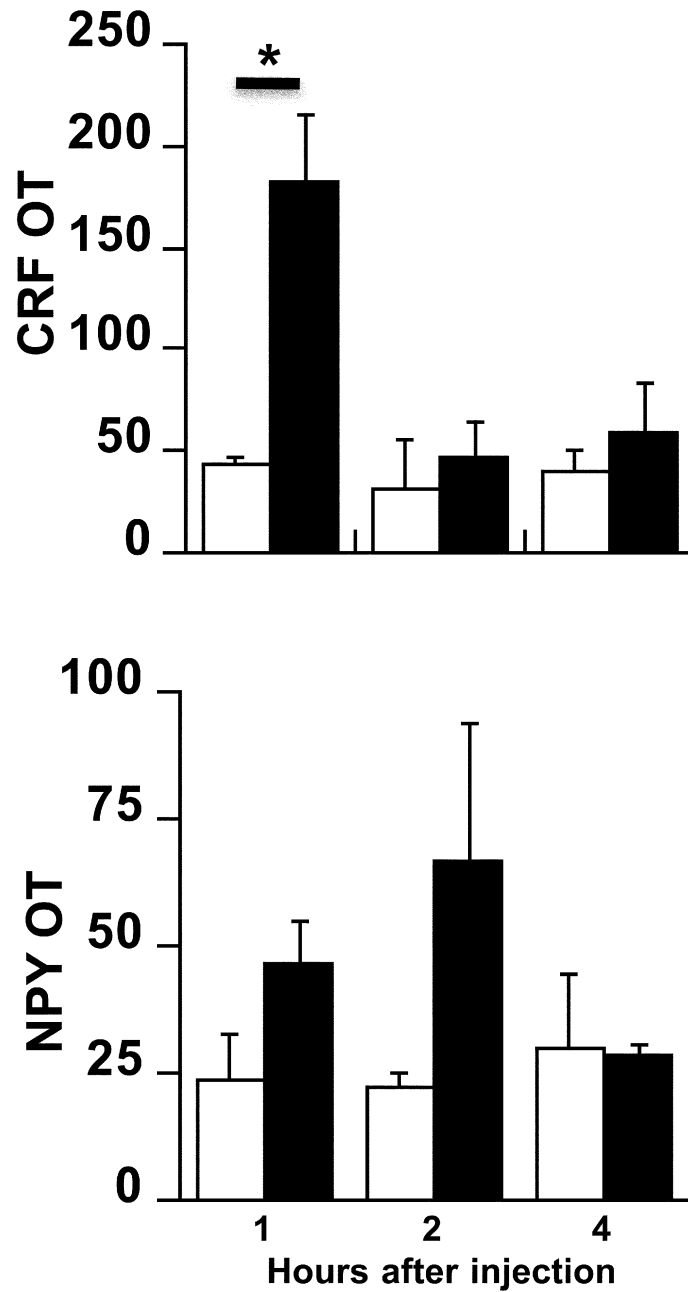
Fig 2. Dark field analysis of silver grains expressed in unit-less values of optical transmission (OT). Top , CRF mRNA levels (ANOVA, p < 0.05 treatment); bottom , NPY mRNA levels (ANOVA, p < 0.05 treatment) following an acute PVN injection of fenfluramine (200 nmol/0.5 \mu l/side). Black bars = fenfluramine; white bars = vehicle; * = p < 0.03 (Fisher's test), n = 4-5 /group.
