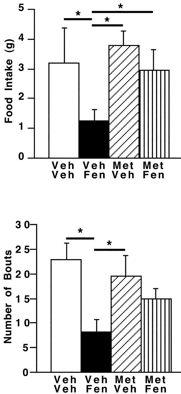
Fig 4. Levels of food intake and feeding bouts following drug administration. Metergoline (MET; 15 nmol/0.5 \mu l/side) or vehicle (VEH) was administered into the PVN just prior to the PVN injection of fenfluramine (FEN; 200 nmol/0.5 \mu l/side) or vehicle. A) Food intake (ANOVA, p < 0.03 , treatment effect) or B) feeding bouts (ANOVA, p < 0.02 ; treatment effect) were measured 1 hour after drug administration. * = p < 0.04 (Fisher's test); n = 4-5 /group.
