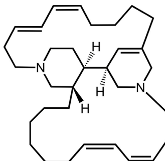
Figure 1. Chemical structure of halicyclamine A.
