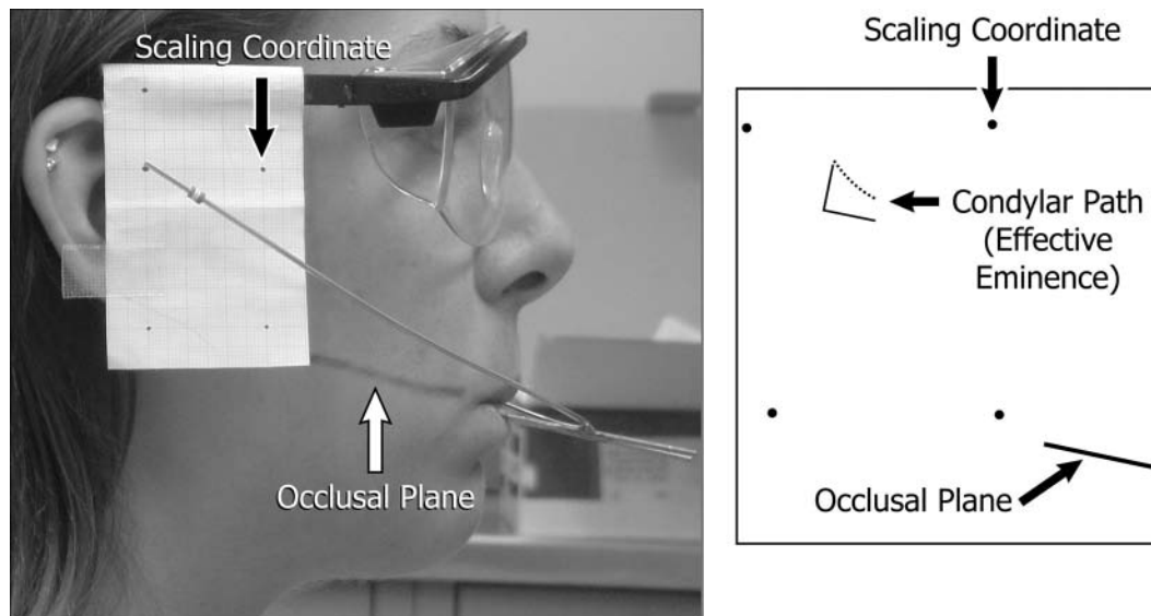
Figure 1. Image of a participant (left) during jaw-tracking and tracing of path of condylar marker (right) relative to occlusal plane. Scaling coordinates are shown as recorded and reproduced in the tracing. Perpendicular lines represent the axis system used in Figs. 2 and 3.
