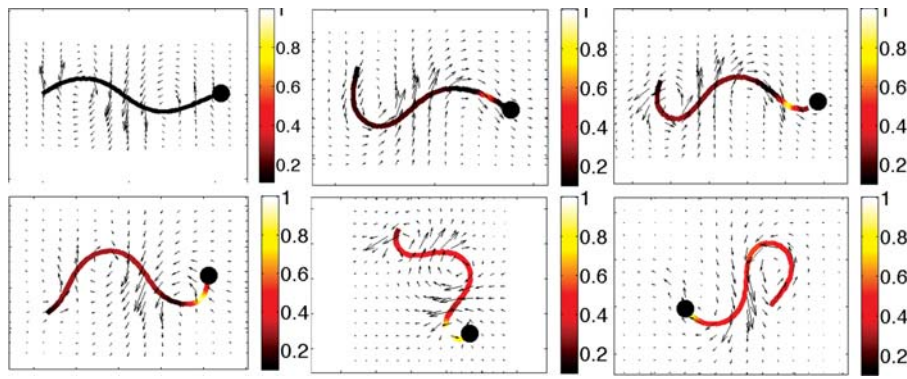
Figure 3 Simulations of a swimming sperm in a 3-dimensional viscous fluid where the CatSper-mediated Ca^{2+} dynamics are accounted for and are coupled to the preferred curvature. The solid black circle denotes the head side of the flagellum. Velocity vectors for the local fluid velocity are depicted in the plane of the beating flagellum and the calcium concentration along the length of the flagellum is shown. After application 8-Br-cAMP, the Ca^{2+} profiles (as in Fig. 2) are determined by the partial differential equations accounting for release of Ca^{2+} from the RNE. These Ca^{2+} concentrations are then used to define a preferred curvature for the flagellar waveform using a modified Hill function for the amplitude. From left to right, top row: t = 0, 1, 2 s and bottom row: t = 4, 6, 8 s. Note how the waveform is modified as the Ca^{2+} concentration increases.
