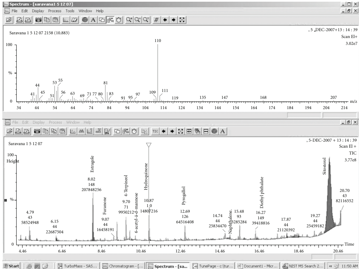
FIGURE 1: GC-MS analysis showing the presence of plant sterols.
