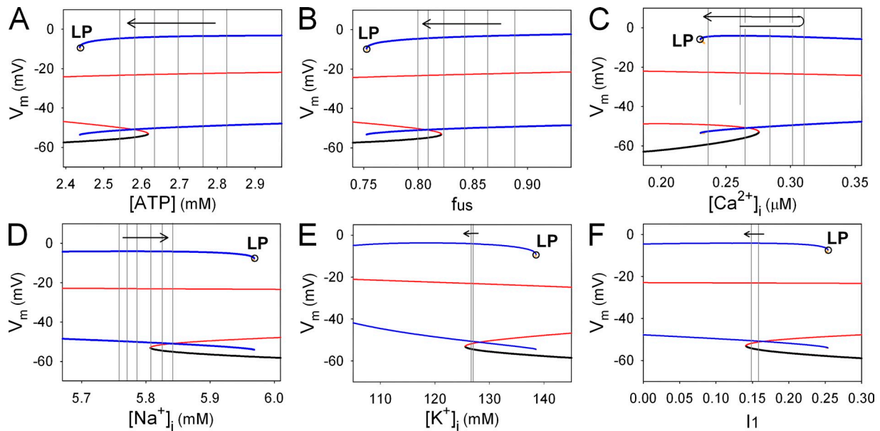
Figure 5. Effects of individual slow variables on the mode change toward termination of the burst. Each bifurcation diagram was obtained by varying single slow variable, [ATP] (A), f_{is} (B), [Ca^{2+}]_i (C), [Na^+]_i (D), [K^+]_i (E), and I_1 (F) as a bifurcation parameter, with the remaining slow variables fixed at their values at 0.9 s before the LP bifurcation (open circles). Stable EPs, unstable EPs, stable LCs, and unstable LCs are indicated by black, red, blue, and yellow lines, respectively. Six gray vertical lines in A–D indicate the values of the corresponding slow variables sampled at an interval of 1 s (from 11 to 16 s in Fig. 4 A). In C, the sequential values of the minimum [Ca^{2+}]_i were sampled. In E and F, two gray lines indicate the corresponding values at 11 and 16 s. Arrows represent the sampling sequence. We confirmed that the bifurcation diagrams were qualitatively the same when slow variables were fixed at different time points during the burst.
