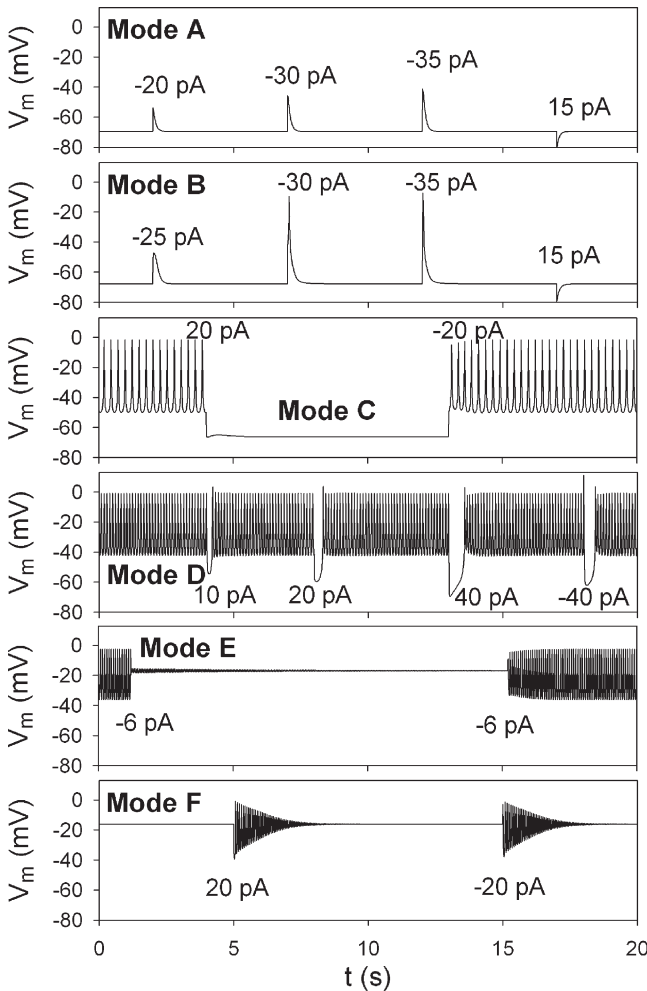
Figure 3. Representative membrane responses to current injections in different modes. The amplitudes of injected current pulses are indicated inside panels. Duration of the pulse was 5 ms, except 15 ms in Mode E. In each panel, a different value of P_{CaV} was used for simulation (units in \text{pA mM}^{-1} ): Mode A, P_{CaV} was 30; Mode B, 45; Mode C, 48.9; Mode D, 60; Mode E, 65; Mode F, 69. The same values were used for the slow variables as in Fig. 2. The time axes were identical for all panels.
