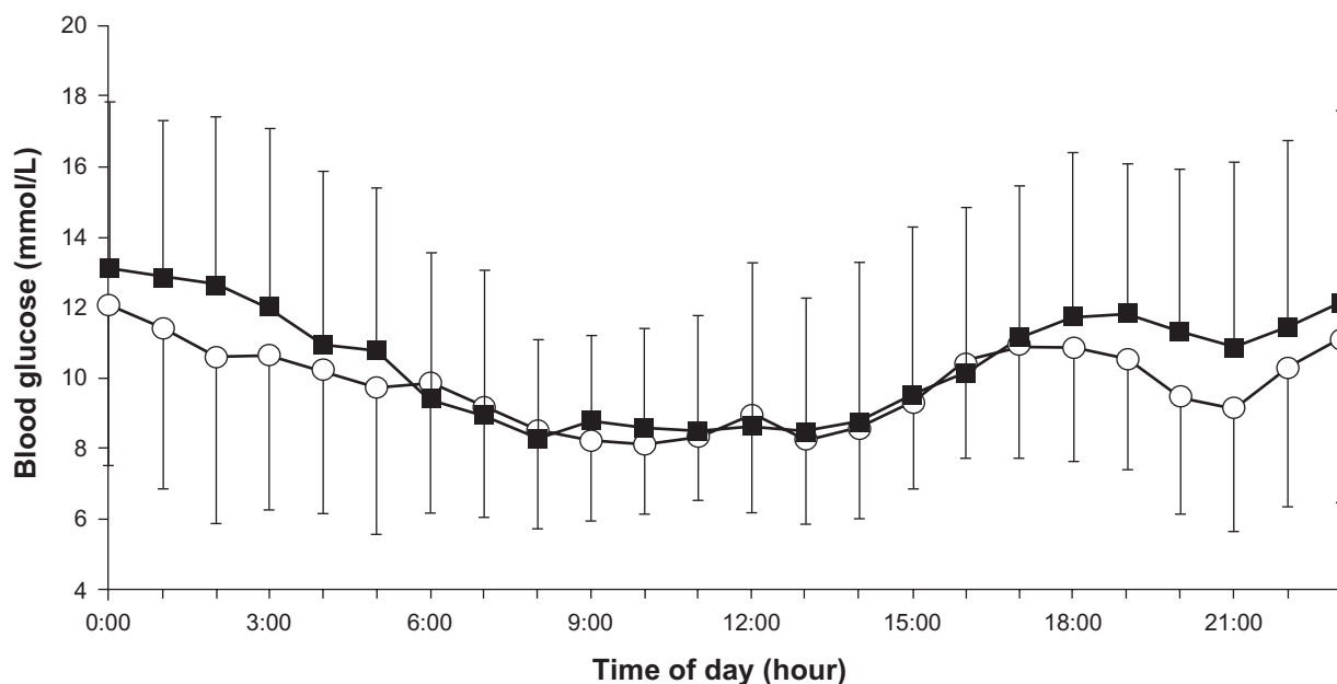
Figure 1 24-hour glucose profiles of day 2 and day 3. Each point represents the mean ± standard deviation of nine patients treated with insulin glargine (O) or detemir (■).
