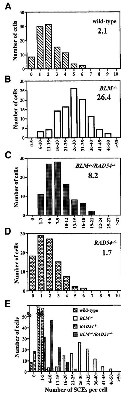
Fig. 5. Histograms of SCE in wild-type, RAD54 -/- , BLM -/- and BLM -/- /RAD54 -/- cells. SCEs in the macrochromosomes were counted. Histograms show the frequency of cells with the indicated number of SCEs per cell. The mean number of SCEs per cell is shown in the upper right corner. (A) Wild-type cells; (B) BLM -/- cells; (C) BLM -/- /RAD54 -/- cells; (D) RAD54 -/- cells; (E) a superimposed figure of (A), (B), (C) and (D) expressed on the same scale.
