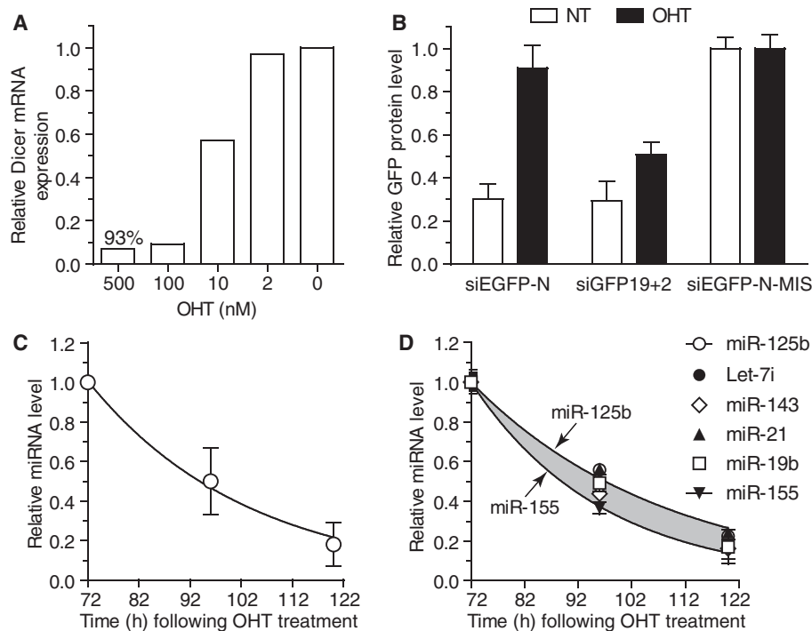
Figure 2. Determination of global miRNA decay. (A) Actively dividing Dicer1 flox/flox ;xCre/Esr1 MEFs were treated overnight with the indicated concentration of OHT, washed with fresh medium and further incubated for 48 h before being harvested for RNA extraction. Wild-type Dicer1 mRNA was quantified by RT-qPCR and reported to the expression of GAPDH . The data are presented relative to that obtained without OHT treatment (condition '0'), are averaged from biological duplicate and are representative of three independent experiments. (B) Actively dividing Dicer1 flox/flox ;xCre/Esr1 GFP MEFs were treated (OHT) or not (NT) overnight with 500 nM OHT, and expanded for a further 48 h before being collected and reverse transfected (on Day 3 following initial OHT addition) with 10 nM of the indicated siRNAs. The cells were further incubated for 24 h and EGFP expression was quantified by fluorescent spectrophotometer [see 'Methods' section and (23)]. The data are averaged from two independent experiments in biological triplicate and are representative of the averaged values obtained for the non-targeting siEGFP-N-MIS sequence for each cell type. siEGFP-N-MIS contains two mismatches in the targeting strand of the siRNA compared to siEGFP-N and both siRNAs are Dicer1 substrates (Supplementary Figure S1C); siGFP19+2 is a Dicer1 product (23). (C and D) Actively dividing Dicer1 flox/flox ;xCre/Esr1 MEFs treated with 500 nM OHT were expanded and collected at Days 3–5 following initial OHT treatment. For each miRNA measured, the levels were reported to that obtained at Day 3 ( T = 72 h following OHT treatment). (C) The average level of 104 miRNAs significantly detected by low-density PCR microarray ('Methods' section and Supplementary Table S1) is shown with fitted exponential regression. (D) Individual miRNA PCRs were carried out on the samples analysed with low-density PCR microarray and biological replicates. Highlighted in grey is the variation of miRNA decay observed between the six miRNAs analysed, and fitted exponential regression is shown for miR-125b and miR-155. The data are averaged from biological triplicate and are representative of three independent experiments. SEM (B and D) and standard deviation (SD) (C) are shown.
