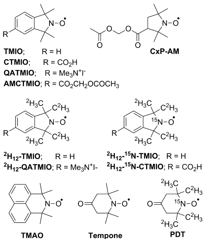
Figure 1. Nitroxides used in this study
