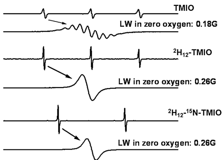
Figure 2. The effect of isotopic labeling on the EPR spectrum of TMIO (1 mM in water) in the absence of \text{O}_2
