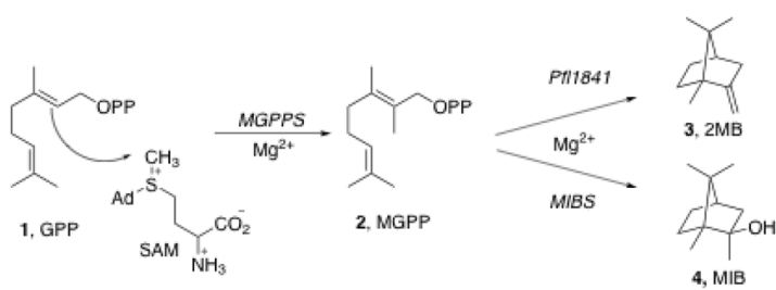
Figure 1. Biosynthesis of 2-methylenebornane (upper pathway) and 2-methylisoborneol (lower pathway).
