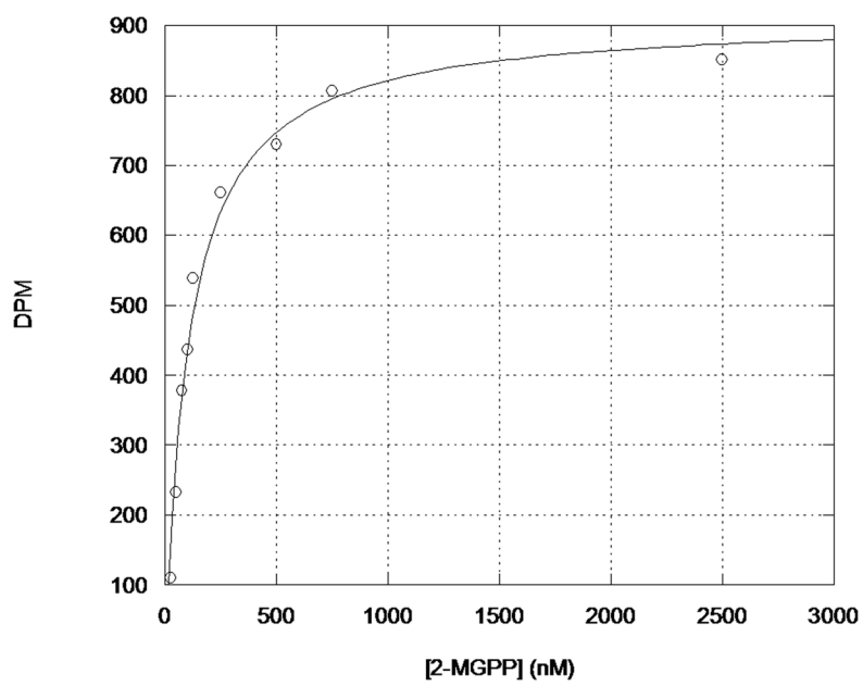
Figure 5. Michaelis-Menten plot of the reaction velocity for the Pfl_1841-catalyzed formation of 2-methylene bornane as a function of the concentration of 2-MGPP.
