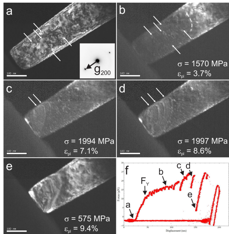
Figure 2. Dark field still images extracted from an in situ TEM compression test of a (100) oriented 118 nm diameter copper pillar irradiated to 0.8 dpa (a-e) and the measured load – displacement data (f)
