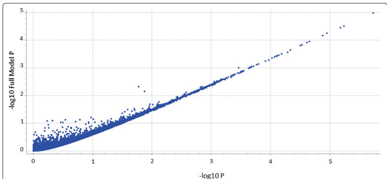
Figure 1 Plot of full vs. reduced model (-log 10 P values). X-axis reduced model including DNA source as covariate. Y-axis full model. 173,662 markers were sorted by (-log 10 P values). The r = 0.95 indicates the equivalence of the buccal and blood derived DNA in the generation of SNP genotypes.
