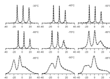
Fig. 3. EPR spectra of 200 \mu\text{M} pdMTSL in degassed sec-butylbenzene collected using magnetic field modulation (dashed line) and NARS (solid line).
