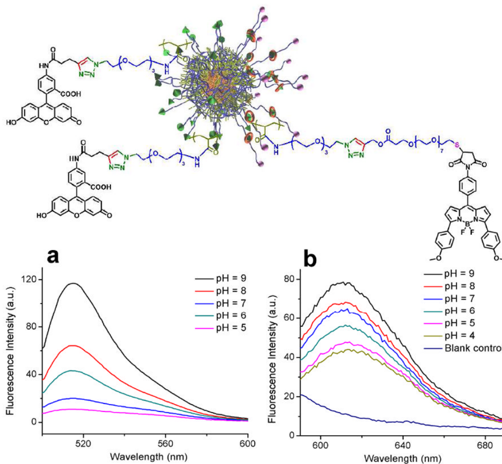
Fig. 3. a, pH-dependent fluorescence spectrum ( \lambda_{\text{ex}} = 488 \text{ nm} ) of JSCKs labeled with alkyne-functionalized fluorescein and thiol-reactive BODIPY 577/618 maleimide, showing the presence of fluorescein. b, pH-dependent fluorescence spectrum ( \lambda_{\text{ex}} = 577 \text{ nm} ), showing the presence of BODIPY 577/618 maleimide. The chemical structures of each of the conjugated dyes are shown above the corresponding spectra.
