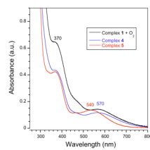
Figure 9. Absorption spectra of 1 + O 2 (black trace), 4 (blue trace), and 5 (red trace) in dichloromethane.
