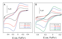
Figure 7. Cyclic voltammograms of 1.0 mM solutions of 1 (A) and 2 (B) in dichloromethane at various scan rates. Tetra- n -butylammonium hexafluorophosphate (0.2 M) was used as the supporting electrolyte. All data were obtained using a platinum working electrode and electrochemical potentials are referenced externally to the ferrocene/ferrocenium couple. Quasi-reversible redox couples at +16 mV and +108 mV were measured for 1 and 2 , respectively, at a scan rate of 100 mV/s.
