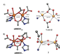
Figure 3. Depiction of the X-ray crystal structures of the diiron sites of sMMOH red (top, left) and sMMOH ox (bottom, left). For structural comparison, synthetic complexes that mimic each protein state are shown on its right. Some relevant bond lengths are provided; the distances shown for 1 and 2 are averaged over the two complexes. Color scheme: iron, orange; nitrogen, blue; oxygen, red; carbon, gray.
