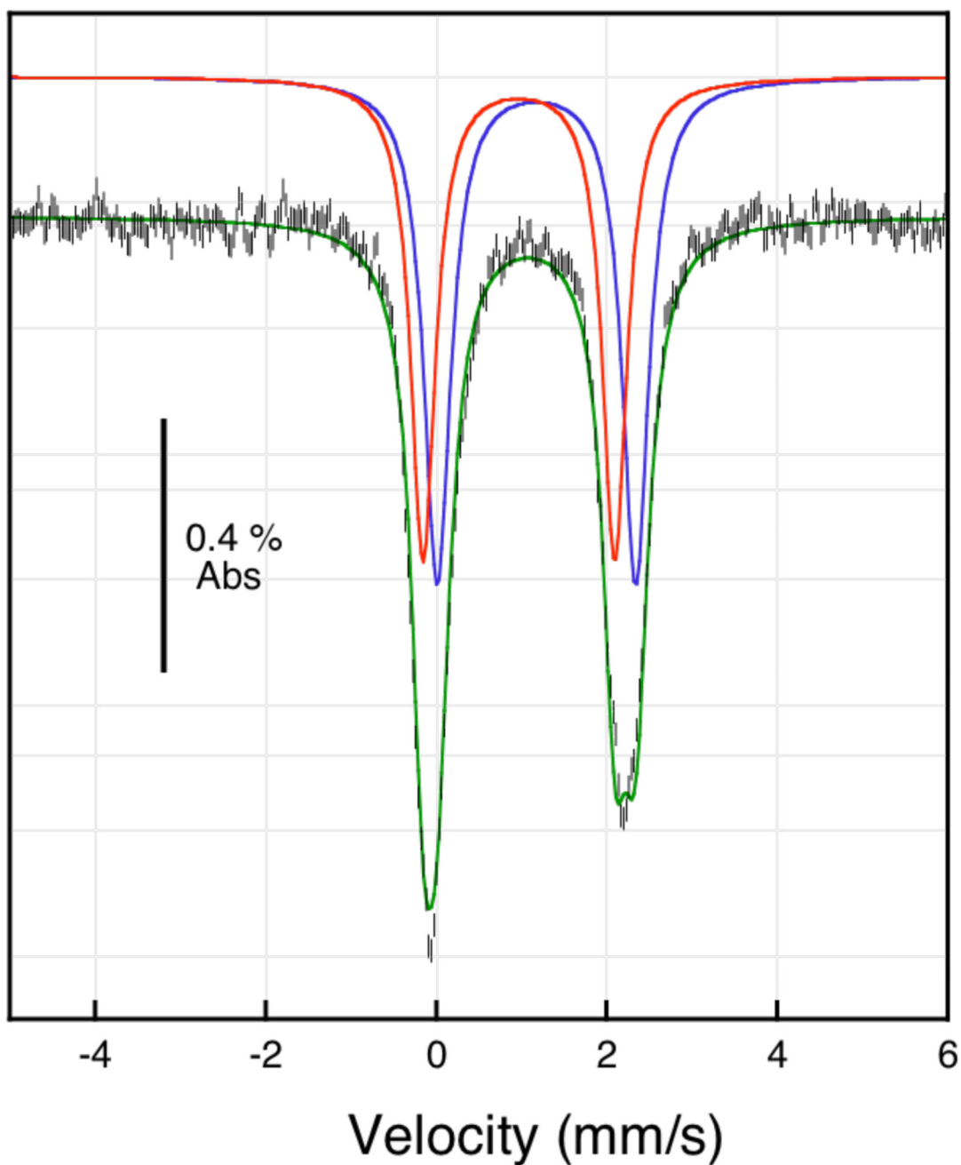
Figure 5. Zero-field ^{57}\text{Fe} Mössbauer spectrum of a polycrystalline sample of [\text{Fe}_2(\text{PIM})(\text{Ph}_3\text{CCO}_2)] (1) at 80 K. The raw data (black hash lines) were fit to two distinct iron sites (green trace). The single site fits are shown as blue and red traces using the following parameters: \delta_1 = 1.18(2) mm/s, \Delta E_{Q1} = 2.33(2) mm/s, \Gamma_{L/R(1)} = 0.38(2) mm/s; \delta_2 = 0.97(2) mm/s, \Delta E_{Q2} = 2.25(2) mm/s, \Gamma_{L/R(1)} = 0.35(2) mm/s.
