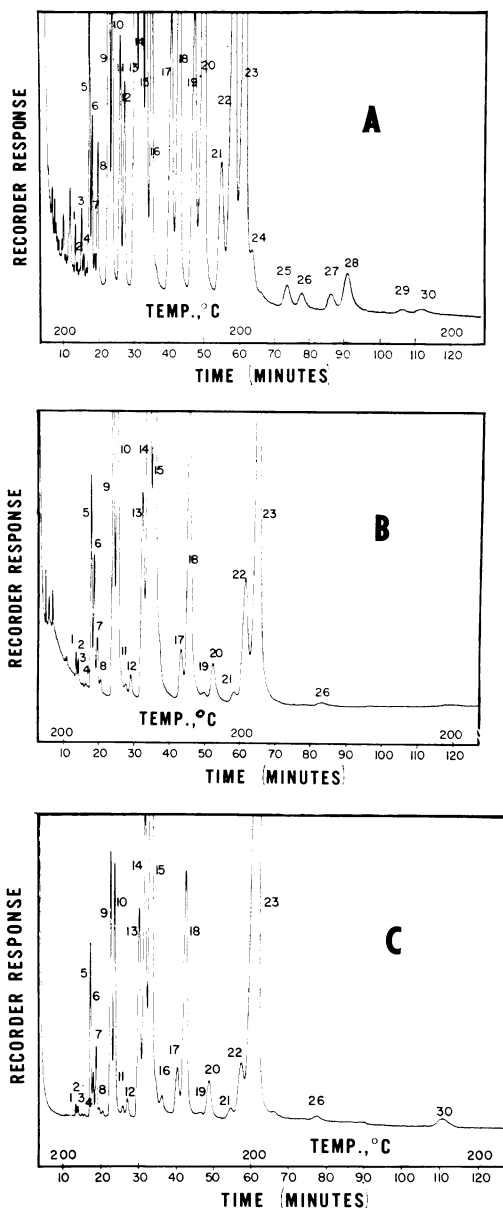
FIG. 2. Gas chromatographic separation of the hydrocarbons of Sarcina lutea on a stainless-steel column (155 meters by 0.076 cm, inner diameter) coated with Igepal. Nitrogen pressure, 933 g/cm 2 ; no split. F & M 810 apparatus equipped with a flame ionization detector. Range, 10°; attenuation 1. Isothermal at 200 C. From 1.5 g of extracted cells, 1/50 of the sample was injected for each preparation. (A) From cells grown in Trypticase Soy Broth. (B) From cells grown in Nutrient Broth. (C) From cells grown in a chemically defined medium.
