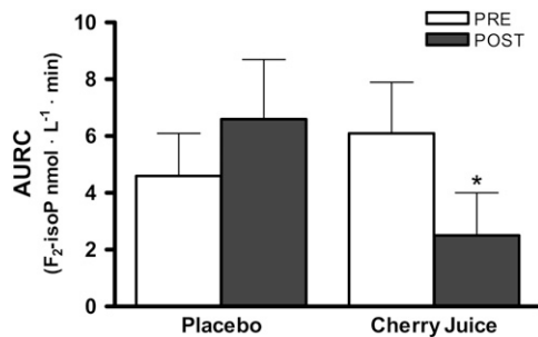
FIGURE 2 Integrated plasma F 2 -isoprostane response to the I/R trial in healthy older adults. Values are means ± SEM, n = 11, calculated as AURC pre- and postplacebo and tart cherry juice intervention. *Pre-post difference compared with pre-post placebo, P < 0.05.
