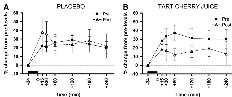
FIGURE 1 Plasma F 2 -isoprostane responses to the I/R trial in healthy older adults. Values are means ± SEM, n = 11, for percent change from baseline levels pre- and postplacebo (A) and tart cherry juice (B). The heavy dark line denotes the time of forearm I/R. The I/R trial increased plasma F 2 -isoprostane levels (main effect of time, P < 0.05). The tart cherry juice intervention decreased the F 2 -isoprostane response to the I/R trial: treatment × trial interaction, P < 0.05, and treatment × trial × time point interaction, P < 0.01.
