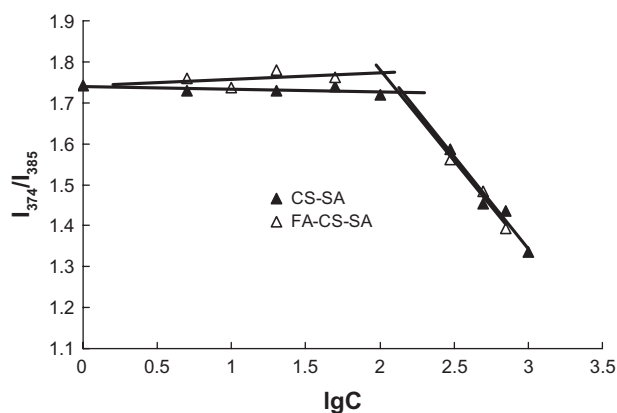
Figure 1 Variation of intensity ratio ( I_1/I_3 ) vs the logarithm of concentration of CS-SA and FA-CS-SA. Unit of concentration was \mu\text{g}/\text{mL} .
