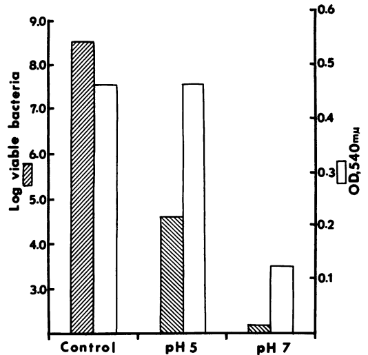
FIG. 4. Effect of pH on bactericidal (hatched bars) and bacteriolytic (open bars) activities of mixtures containing H_2O_2 , AA, and Lys at concentrations indicated in the text. The control tubes contained the bacteria in buffer alone. Incubation was at 37 C for 30 min.
