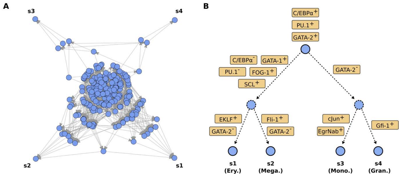
Figure 3. Systems dynamics of the myeloid differentiation model. (A) State-transition graph of the Boolean model with dynamical trajectories. Each node represents a Boolean state of the system where each player is either 'on' or 'off'. Each edge stands for a transition between two states induced by the application of a single Boolean update rule. The shown subgraph is calculated from a central early hematopoietic state and comprises 232 nodes with 789 links. The visualization emphasizes the existence of four attractors reachable from the early state, and the hierarchical structuring of the state space with two pairs of attractors (s1/s2 and s3/s4, respectively) that share a common attractor basin. The distance of a state from the attractor in the graph corresponds to the number of necessary update steps. (B) Interpretation of the state space in the context of myeloid differentiation. We observe a hierarchical partitioning with subsequent splits between the GM and MegE lineages, followed by splits of the granulocyte and monocyte lineages, and the erythrocyte and megakaryocyte lineages, respectively. Arrows in the diagram represent expression changes on the respective branch of the differentiation tree. doi:10.1371/journal.pone.0022649.g003
