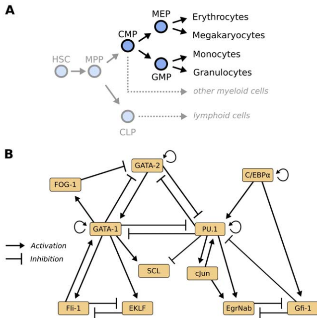
Figure 1. A regulatory model of myeloid differentiation. (A) Hematopoietic stem cell (HSC) differentiation consists of a series of switch-like decisions. We here focus on differentiation into four myeloid cell types and omit other myeloid cells and the lymphoid branch (greyed out). For a detailed discussion of the different progenitor cell types, we refer the reader to [1]. Abbreviations: MPP, multipotent progenitor; CMP, common myeloid progenitors; MEP, megakaryocyte-erythrocyte progenitor; GMP, granulocyte-monocyte progenitor; CLP, common lymphoid progenitor. (B) Literature-derived gene regulatory network for 11 myeloid players previously reported to be pivotal for the lineage decisions in myeloid differentiation (compare Text S1). Note that this visualization does not contain explicit Boolean update rules. Specifically, it is not apparent from the graph visualization alone whether multiple regulatory inputs are combined using AND or OR logic, which can make substantial differences for the resulting Boolean dynamics. doi:10.1371/journal.pone.0022649.g001
