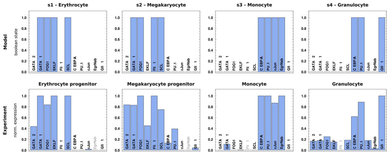
Figure 4. Comparison of Boolean states (top) with normalized mRNA expression profiles (bottom) for the 11 players of our model (see text for a detailed discussion). We observe a good agreement between model prediction and measured mRNA expression. Note that we excluded non-differentially expressed genes with a maximum fold change smaller than 2 in all samples of the respective study (EgrNab in Pronk et al. [51] and Flt-1 in Chambers et al. [50], greyed out). For a discussion of the mismatch between prediction and data for GATA-2, see main text.
