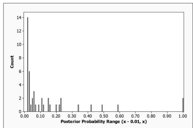
(b) Prior = 0.0001
