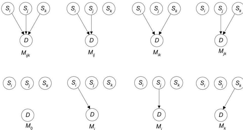
Figure 5. A 3-SNP model and its competing models. doi:10.1371/journal.pone.0022075.g005
