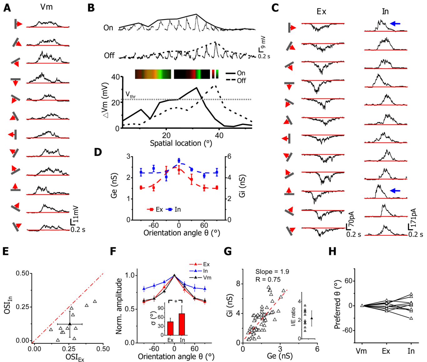
Figure 2. Orientation tunings of excitatory and inhibitory synaptic inputs to simple cells (A) Vm responses to single drifting bars of various orientations. Red lines indicate the level of resting membrane potential. (B) One-dimensional RF of Vm responses to flashing bars of preferred orientation. Middle, average Vm responses evoked by bright (On) and dark (Off) bars at different spatial locations. Bar width was 3.5^\circ . The solid and dash curves depict the spatial tuning curves (i.e. the envelope of peak response amplitudes) for On and Off responses, respectively. Bottom, superimposed On and Off spatial tuning curves. An arbitrary spike threshold ( V_{thr} ) of 22 mV above the resting level was applied. Inset, color maps for On (red) and Off (green) Vm responses before (left) and after (right) subtracting the spike threshold. The brightness of colors represents the peak amplitude of membrane depolarization. (C) Average excitatory (Ex) and inhibitory (In) currents evoked by bars of various orientations. (D) Orientation tuning curves for excitatory (red) and inhibitory (blue) conductances in the cell, fitted with a Gaussian function (dash curve). Error bar = SEM. (E) Relationship between OSI_{In} and OSI_{Ex} . (F) Normalized amplitude vs. orientation angle \theta ( ^\circ ). Inset: \sigma ( ^\circ ) for Ex and In. * indicates significance. (G) G_i (nS) vs. G_e (nS). Slope = 1.9, R = 0.75 . Inset: I/E ratio. (H) Preferred \theta ( ^\circ ) for Vm, Ex, and In.
