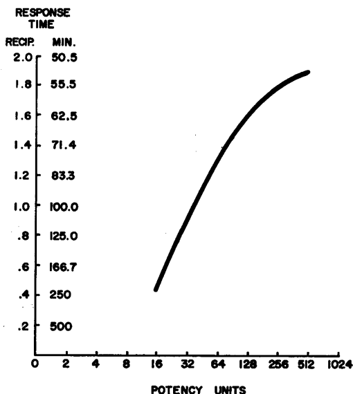
FIG. 1. Regression of reciprocal response time of Fischer rats on \log dose of anthrax toxins expressed in potency units.
