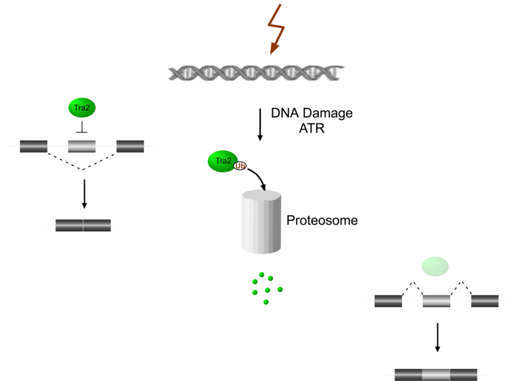
Fig.1. Regulated protein turnover as a means to control alternative splicing
