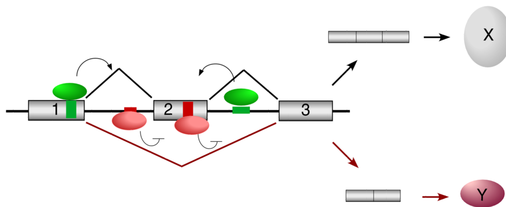
Figure I. Reciprocal regulation of alternative splicing by activator and repressor proteins
