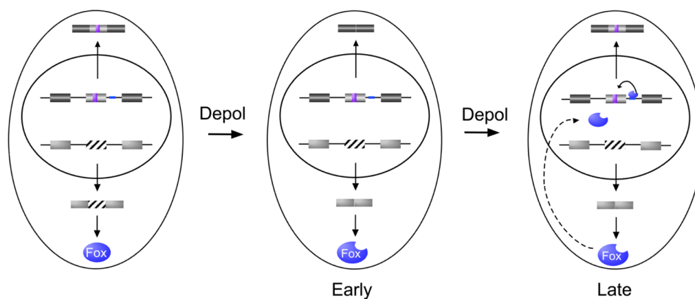
Fig. 4. A feedback loop in signal-induced alternative splicing
