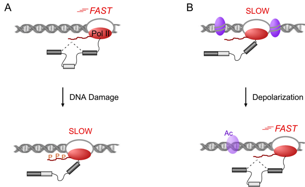
Fig. 3. Signal-induced changes in Pol II processivity regulate cotranscriptional splicing In the kinetic coupling model, alternative splicing can be regulated by the speed of RNA polymerase II (Pol II; red oval) such that a slower polymerase leaves the spliceosome more time to recognize exons with suboptimal splice sites (light grey box), thus increasing inclusion. A) A model for DNA damage-induced alternative splicing of several apoptotic regulators, showed that phosphorylation (P) within the C-terminal domain (CTD, red wavy line) of Pol II leads to reduced Pol II speed and changed patterns of alternative splicing 40 . B) Another mechanism to change Pol II processivity has been seen in neurons. Depolarization leads to loosening of the chromatin structure by changing the acetylation (Ac) of specific histones (purple ovals). This allows for increased Pol II elongation rates and leads to a consistent change in NCAM1 alternative splicing 41 .
