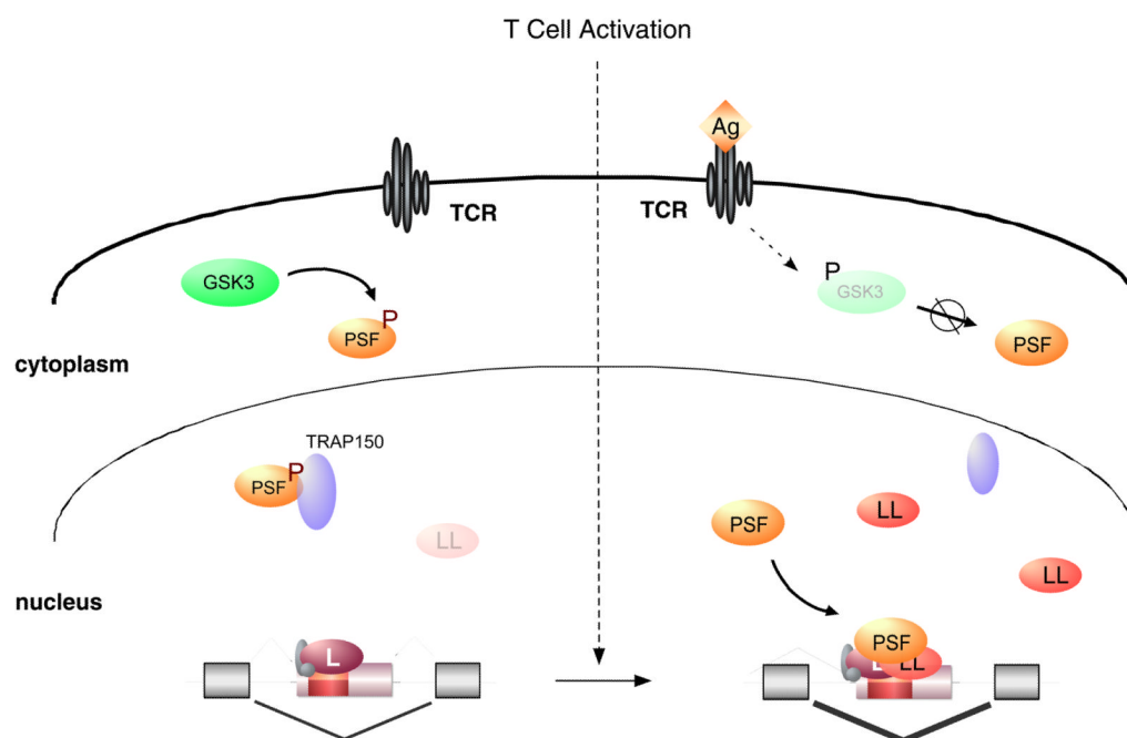
Fig. 2. Altered protein–protein interactions and induced protein expression regulate CD45 alternative splicing during T cell activation
