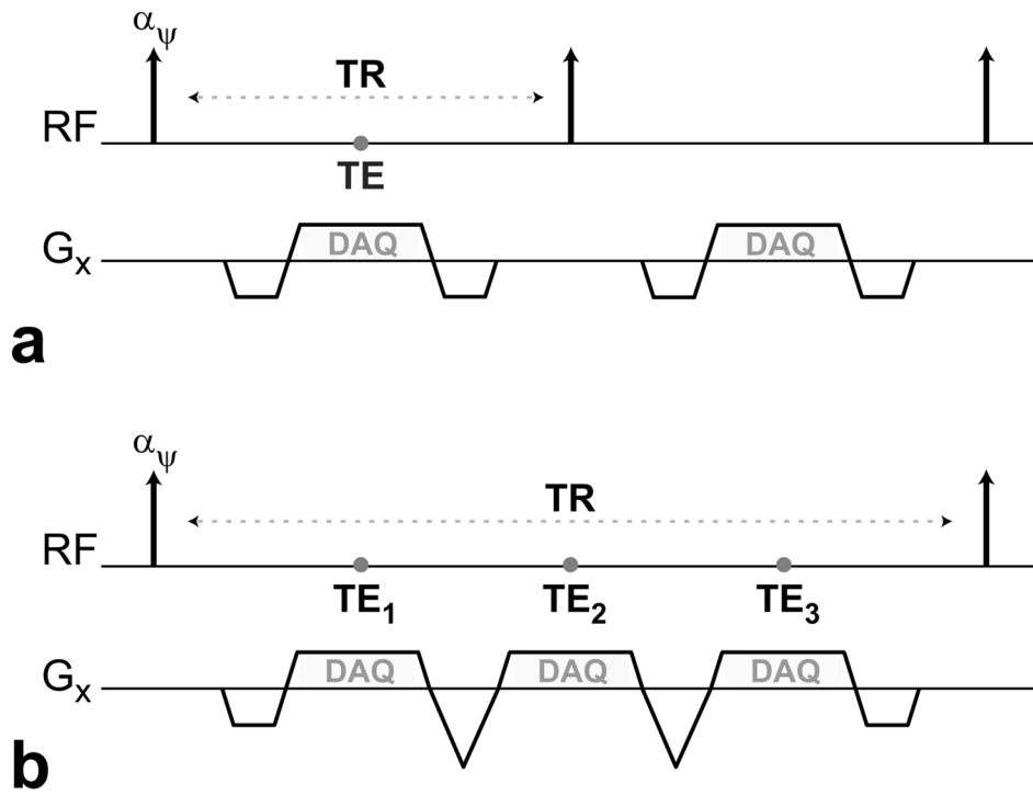
Figure 2. Diagrams showing the RF excitations and the readout gradient waveforms of two bSSFP sequences. a: A single echo is acquired per TR. b: A multiecho flyback acquisition is performed each TR, where the gradients for all three echoes have the same polarity.
