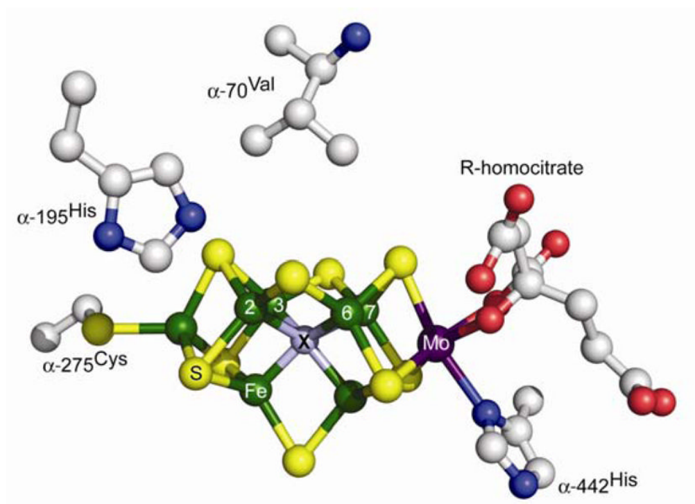
Fig 1. Structure of FeMo-co showing Fe green, Mo purple, S yellow, X, grey.
