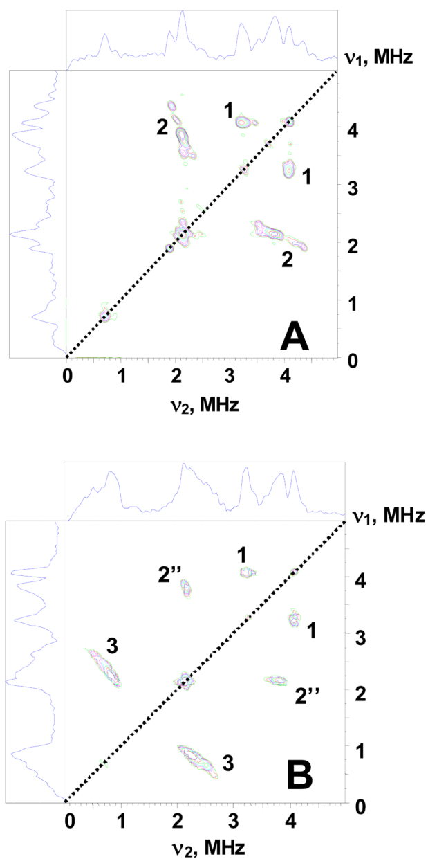
Figure 7. Contour presentations of the ^{14,15}\text{N} HYSORE spectra of the l(\text{N}_2\text{H}_4) intermediate with ^{14}\text{N}_2\text{H}_4 ( A ) and ^{15}\text{N}_2\text{H}_4 ( B ) (magnetic field 345.9 mT ( ^{14}\text{N}_2\text{H}_4 ) and 346.0 mT ( ^{15}\text{N}_2\text{H}_4 ), time between first and second pulses \tau=136 ns, microwave frequency 9.702 GHz ( ^{14}\text{N}_2\text{H}_4 ) and 9.707 GHz ( ^{15}\text{N}_2\text{H}_4 ).
