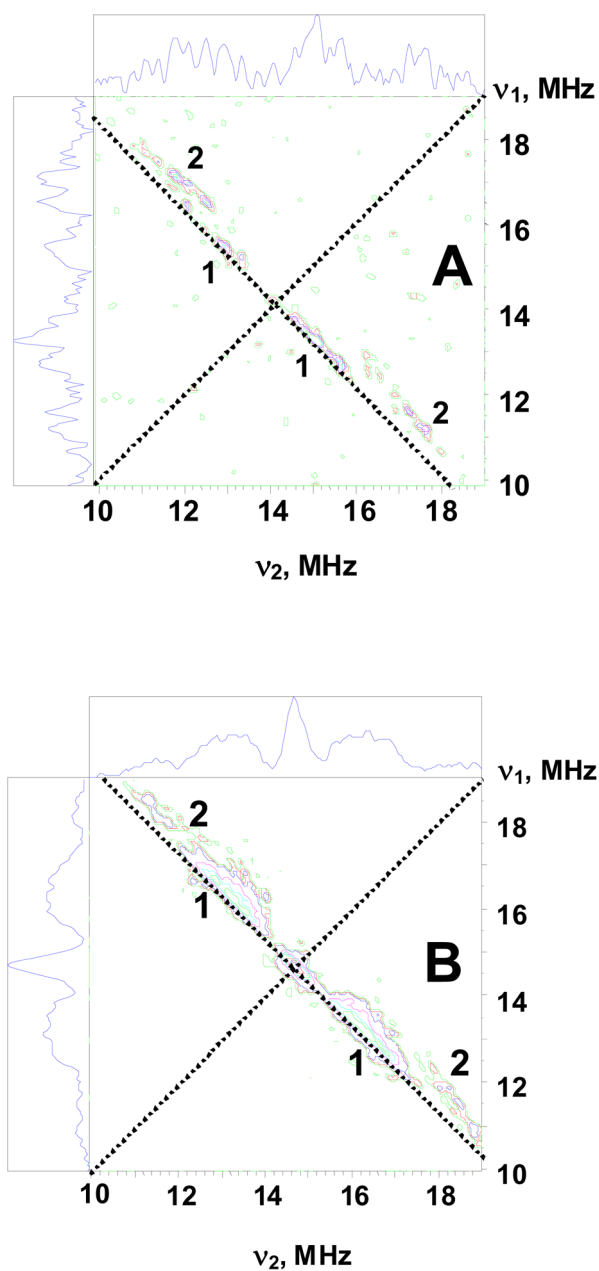
Figure 4. Contour presentations of the ^1\text{H} HYSCORE spectra of the l(\text{N}_2\text{H}_4) intermediate (magnetic field 332.0 mT (A) and 345.0 mT (B), time between first and second pulses \tau=136 ns, microwave frequency 9.6982 GHz).
