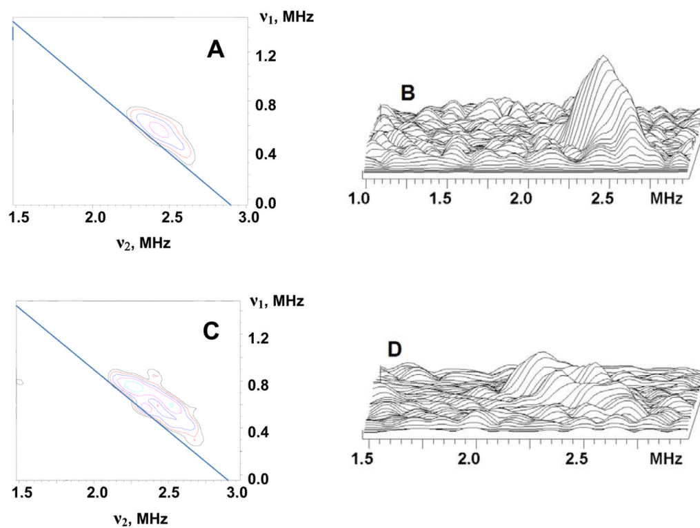
Figure 8. Contour (A, C) and stacked (B, D) presentations of the cross-features 3 from the HYSORE spectra of the l(^{15}\text{N}_2\text{H}_4) intermediate (magnetic field 329.5 mT (A, B) and 332.3 mT (C, D), time between first and second pulses \tau=136 ns, microwave frequency 9.7034 GHz (A, B) and 9.7057 GHz (C, D)).
