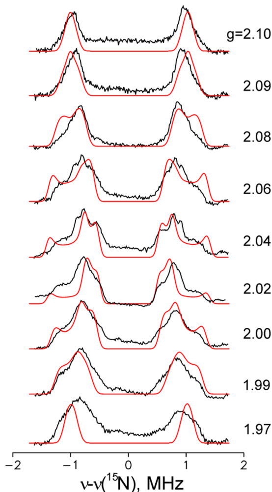
Figure 5. (A) Comparison of 35 GHz ReMims pulsed ^{15}\text{N} ENDOR spectra of intermediates trapped during turnover of the \alpha -70 ^{\text{Ala}}/\alpha -195 ^{\text{Gln}} MoFe protein with ^{15}\text{N}_2\text{H}_4 , ^{15}\text{N}_2\text{H}_4 , and ^{15}\text{NH}=\text{N}-\text{CH}_3 (denoted ^{15}\text{MD} ). (B) 2D Field-Frequency plot of 35 GHz pulsed ^{15}\text{N} ENDOR spectra of l(^{15}\text{N}_2\text{H}_4) intermediate. Conditions: microwave frequency, 34.82 GHz; ReMims sequence, \pi/2 = 30 ns, \tau_1 = 200 ns; RF 40 \mu\text{s} ; repetition time, 10 ms; 500–950 scans; temperature, 2 K. Spectral baselines were corrected by simple subtraction if needed. Simulation (red) parameters: g = [2.09, 2.015, 1.98] , hyperfine tensor A = [1.0, 2.8, 1.5] MHz, Euler angles \phi = 50^\circ , \theta = 60^\circ , \psi = 55^\circ with respect to g-frame.
