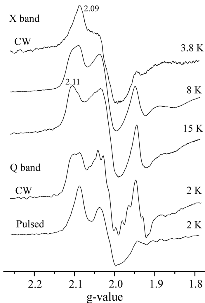
Fig 2. EPR spectra of intermediate I ( l (N 2 H 4 )) detected by various techniques. Conditions for CW X-band: microwave frequency, 9.38 GHz; microwave power, 10 mW; modulation amplitude, 7 G; time constant, 160 ms; field sweep speed, 20 G/s. Conditions for CW Q-band: microwave frequency, 35.08 GHz; microwave power, 32 \mu W; modulation amplitude 4 G; time constant, 128 ms; field sweep speed, 17 G/s. Conditions for pulsed Q-band: microwave frequency, 34.79 GHz; Mims sequence, \pi/2 = 50 ns, \tau = 600 ns; repetition time 10 ms, 50 shots/point; field sweep speed, 8 G/s.
