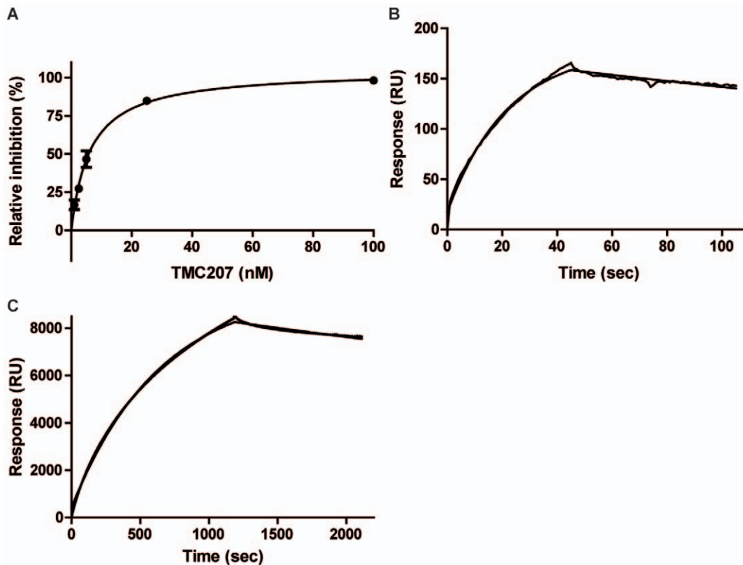
Figure 5. TMC207 binds to a defined binding site in ATP synthase. (A) The dose-dependency of ATP synthesis inhibition by TMC207 in inverted membrane vesicles of Mycobacterium smegmatis was fitted with a one-site binding hyperbola ( Y = 104.9X/6.3+X , R^2 > 0.99 ) (B) Binding of purified ATP synthase subunit c from Mycobacterium tuberculosis to an amine analog of TMC207 linked onto a BIAcore chip was fitted using mono-exponential binding models (Association = Req*(1 - \exp(-1*53737X)) and Dissociation = 165.654*\exp(-1*0.002295*(X-45)) , R^2 > 0.99 ) and (C) Binding of purified ATP synthase from Bacillus PS3 to an amine analog of TMC207 linked onto a BIAcore chip was fitted using mono-exponential binding models (Association = Req*(1 - \exp(-1*153.7X)) and Dissociation = 8575.97*\exp(-1*0.0001030*(X-1187)) , R^2 > 0.99 ). doi:10.1371/journal.pone.0023575.g005
