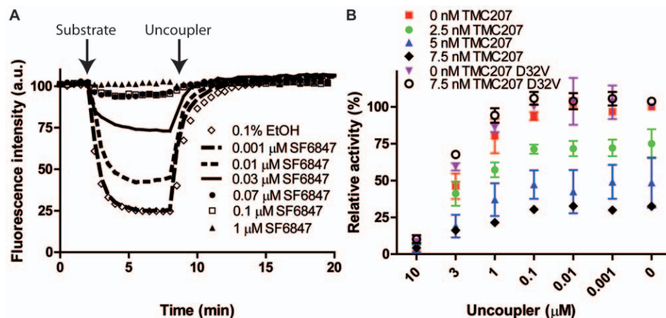
Figure 2. ATP synthesis inhibition by TMC207 at low proton motive force. (A) Inverted membrane vesicles from Mycobacterium smegmatis were diluted to 0.18 mg/ml in buffer containing 2 \mu\text{M} ACMA. To detect the proton motive force, quenching of ACMA fluorescence was investigated after addition of 5 mM succinate in the presence of increasing concentrations of the uncoupler SF6847. At the indicated time point, 1 \mu\text{M} of uncoupler SF6847 was added as control to collapse the proton gradient. (B) ATP synthesis by membrane vesicles of M. smegmatis (1 mg/ml) was measured in the presence of TMC207 and varying concentrations of uncoupler SF6847 to modulate the proton motive force. Samples were incubated at 37°C for 1 h in the presence of an ADP-regenerating system, and produced ATP was quantified spectrophotometrically by monitoring oxidation of glucose-6-phosphate with \text{NADP}^+ . As a control, 100 \mu\text{M} DCCD was added. doi:10.1371/journal.pone.0023575.g002
