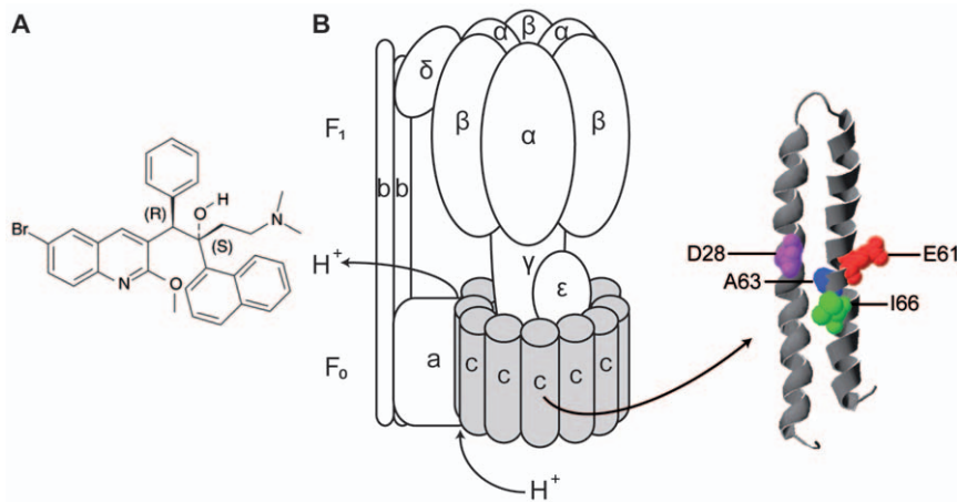
Figure 1. TMC207 and its target mycobacterial ATP synthase. (A) Structure formula of TMC207. (B) ATP synthase subunit composition with subunit c in grey. A homology model of a subunit c monomer from Mycobacterium tuberculosis is shown enlarged. The acidic residue Glu61, essential for proton transport, is depicted in red. Point mutations that influence mycobacterial sensitivity for TMC207 are indicated in colour. doi:10.1371/journal.pone.0023575.g001
