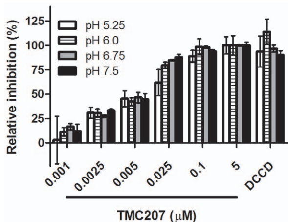
Figure 3. Effect of TMC207 on mycobacterial ATP synthesis at low pH. ATP synthesis in the presence of TMC207 and varying external pH values was measured for Mycobacterium smegmatis inverted membrane vesicles (1 mg/ml). Samples were incubated at 37°C for 1 h in the presence of an ADP-regenerating system, and produced ATP was quantified spectrophotometrically by monitoring oxidation of glucose-6-phosphate with NADP^+ . As a control, 100 \mu M DCCD was added.
