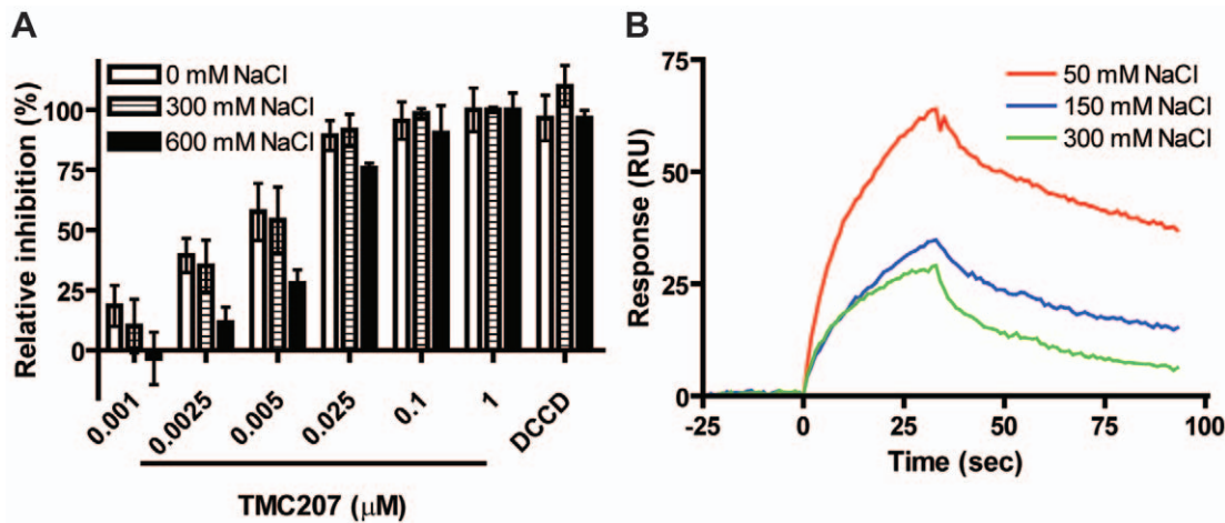
Figure 4. Electrostatic interactions are important for binding of TMC207. (A) ATP synthesis in the presence of TMC207 and increasing sodium chloride concentrations was measured for inverted membrane vesicles of Mycobacterium smegmatis (1 mg/ml). Samples were incubated at 37°C for 1 h in the presence of an ADP-regenerating system, and produced ATP was quantified spectrophotometrically by monitoring oxidation of glucose-6-phosphate with NADP + . As a control, 100 μM DCCD was added. (B) BIAcore binding studies. Purified subunit c from wild-type Mycobacterium tuberculosis was injected onto a chip with immobilized amine analog of TMC207 in the presence of 50, 150, and 300 mM NaCl at 37°C. doi:10.1371/journal.pone.0023575.g004
